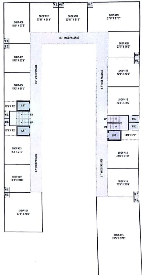
4 th FLOOR PLAN
