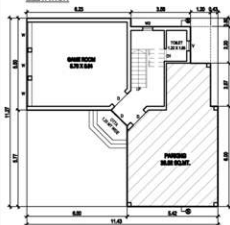
CLUB HOUSE IN COMMON PLOT-4H GROUND FLOORPLAN
