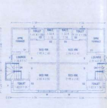
A - FIRST FLOOR
