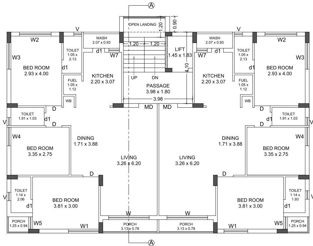
TYPICAL FLOOR PLAN 1st floor to 5th floor (Scale:1:100)
