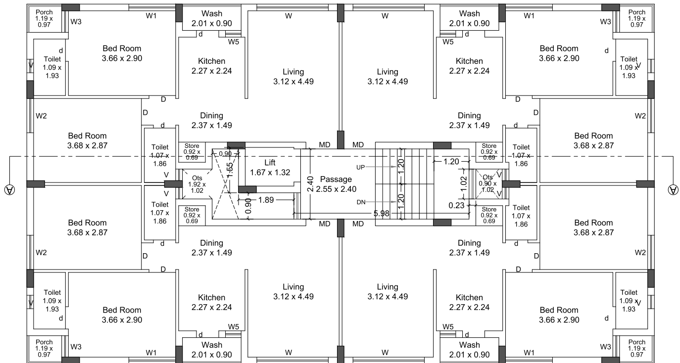
BUILDING - B
