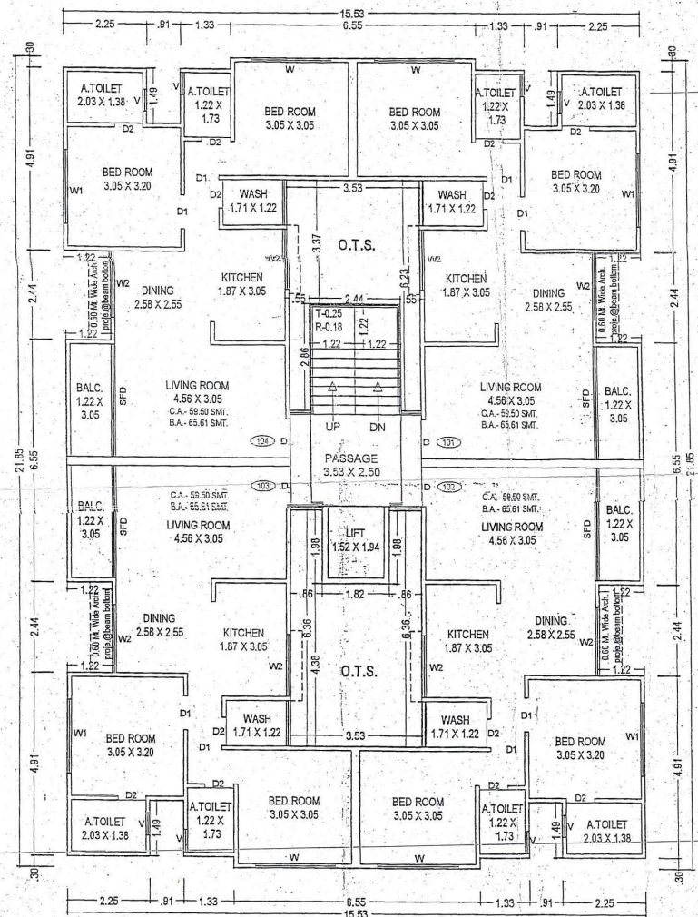
TYPIACL FLOOR PLAN (1ST TO 5TH)
