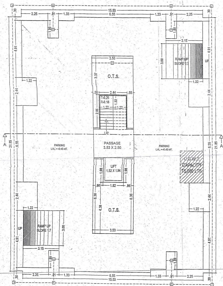
GROUND FLOOR PLAN (PARKING)
