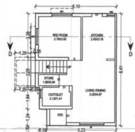
GROUND FLOOR PLAN D-TYPE B.A. = 50.45 SQ.MT. SCALE = 1:100
