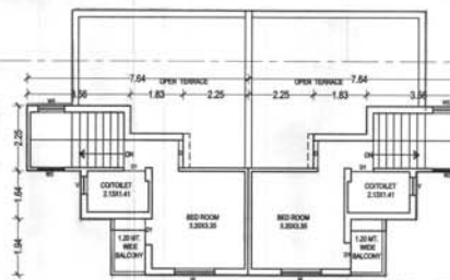
FIRST FLOOR PLAN F.S.I. = 27.50 SQ.MT.
