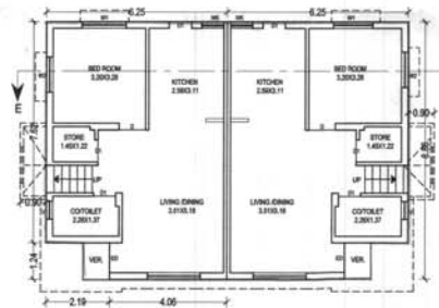
GROUND FLOOR PLAN E-TYPE B.A. = 52.66 SQ.MT. SCALE = 1:100
