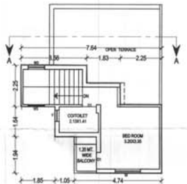
FIRST FLOOR PLAN F.S.I. = 27.50 SQ.MT.
