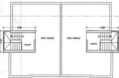
FIRST FLOOR PLAN F.S.I. = 10.49 SQ.MT.
