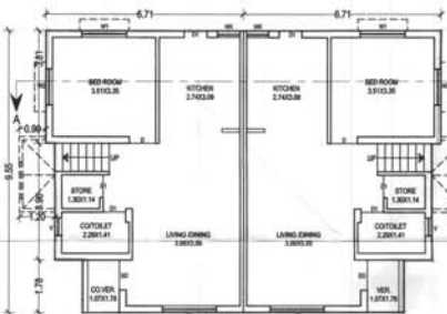
GROUND FLOOR PLAN A-TYPE B.A. = 60.61 SQ.MT. SCALE = 1:100
