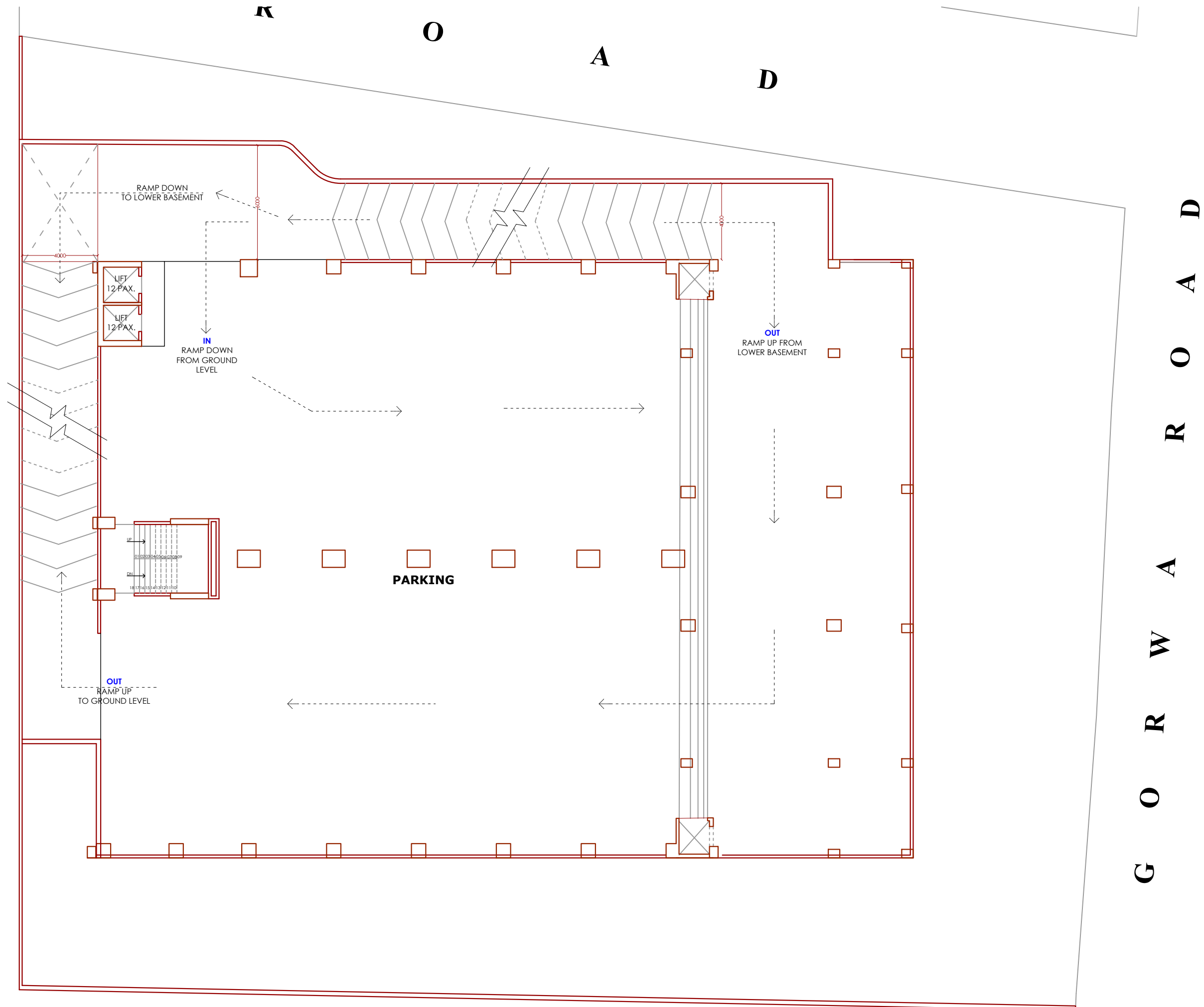
UPPER BASEMENT LAYOUT
