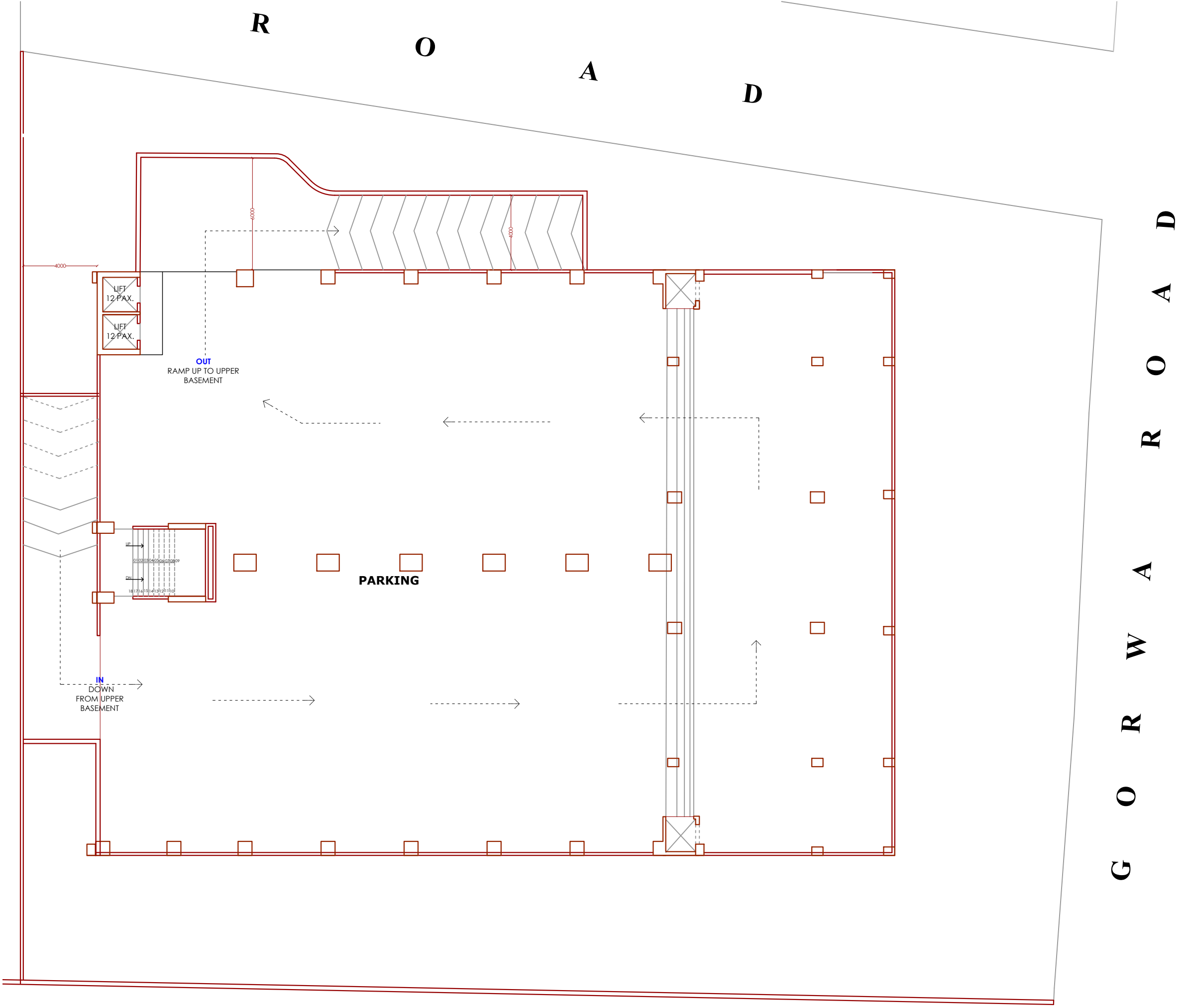
LOWER BASEMENT LAYOUT
