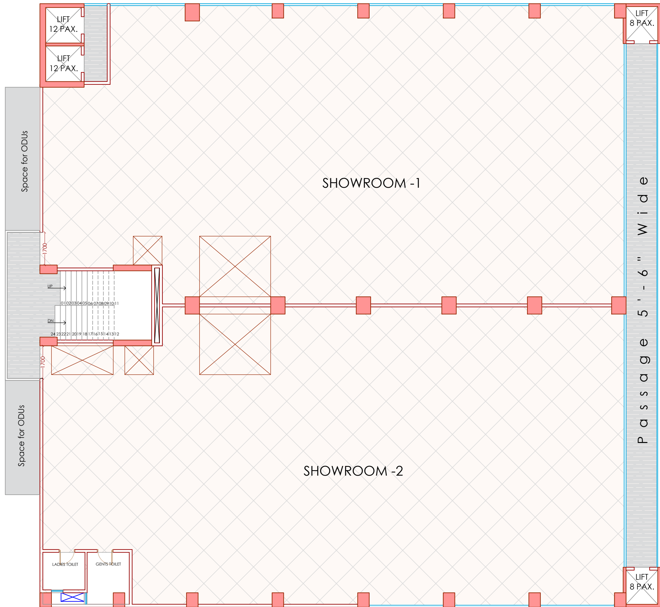
1ST & 2ND FLOOR LAYOUT
