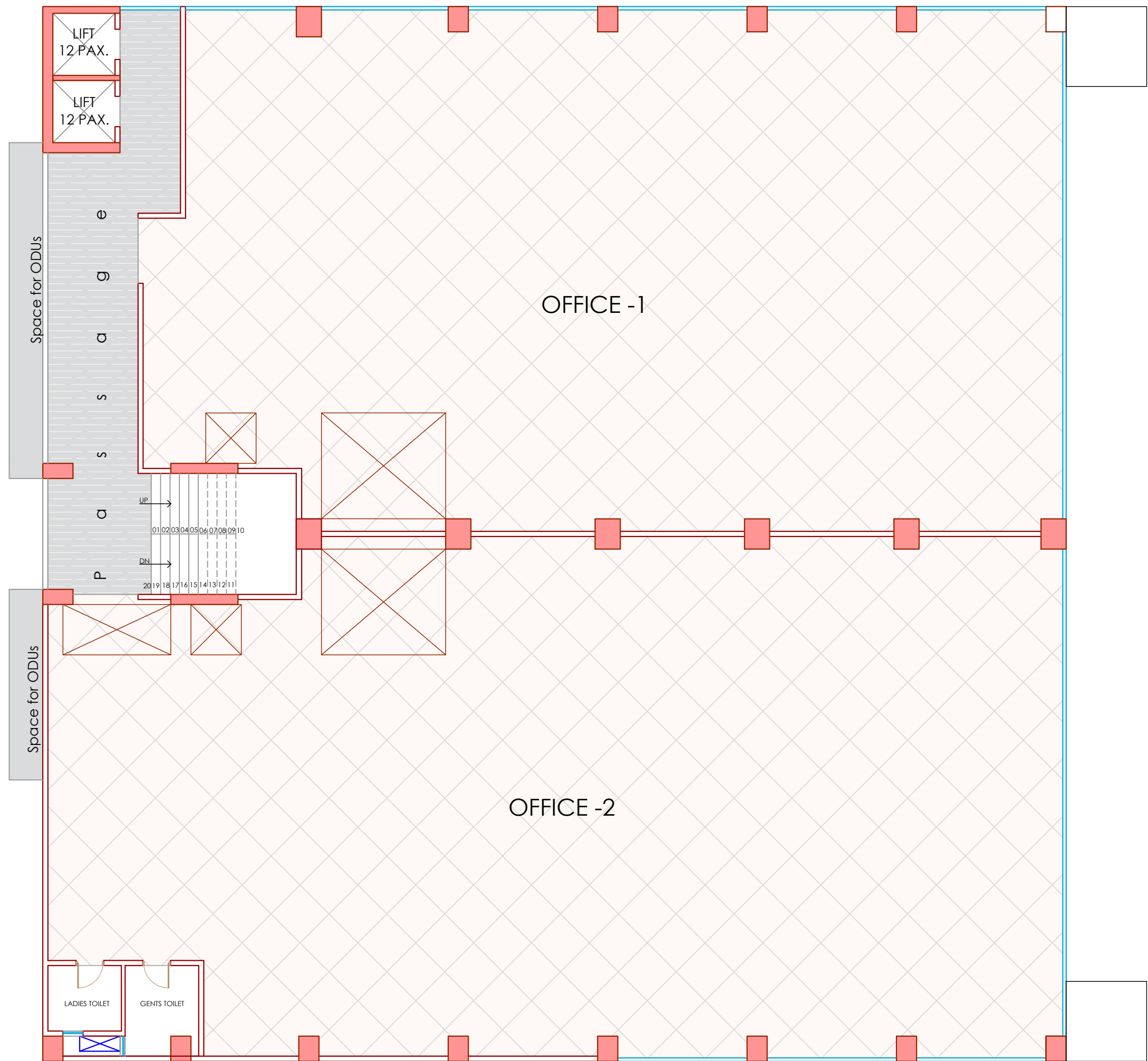
3RD TO 6TH FLOOR LAYOUT
