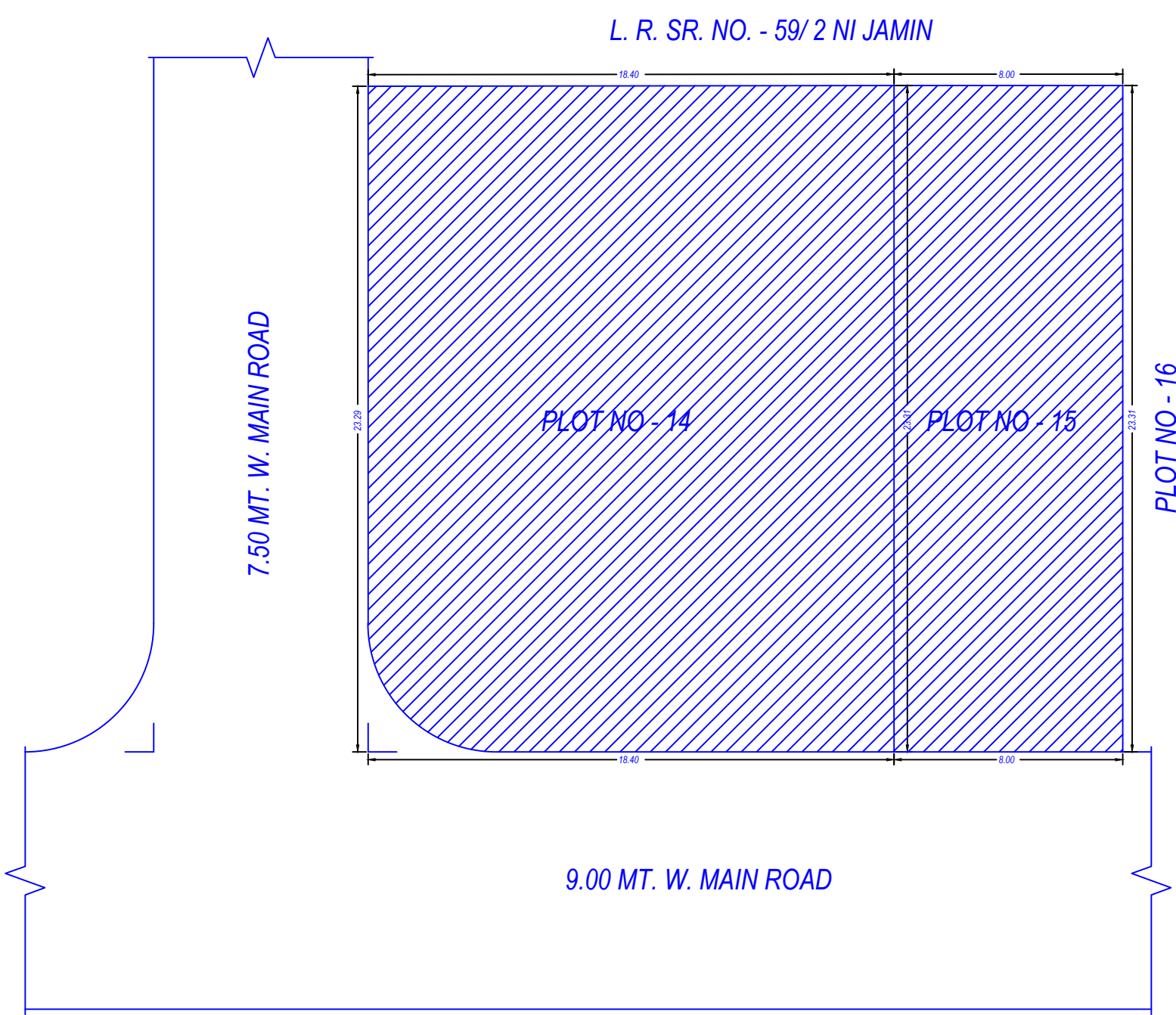
LAYOUT PLAN 1:200
