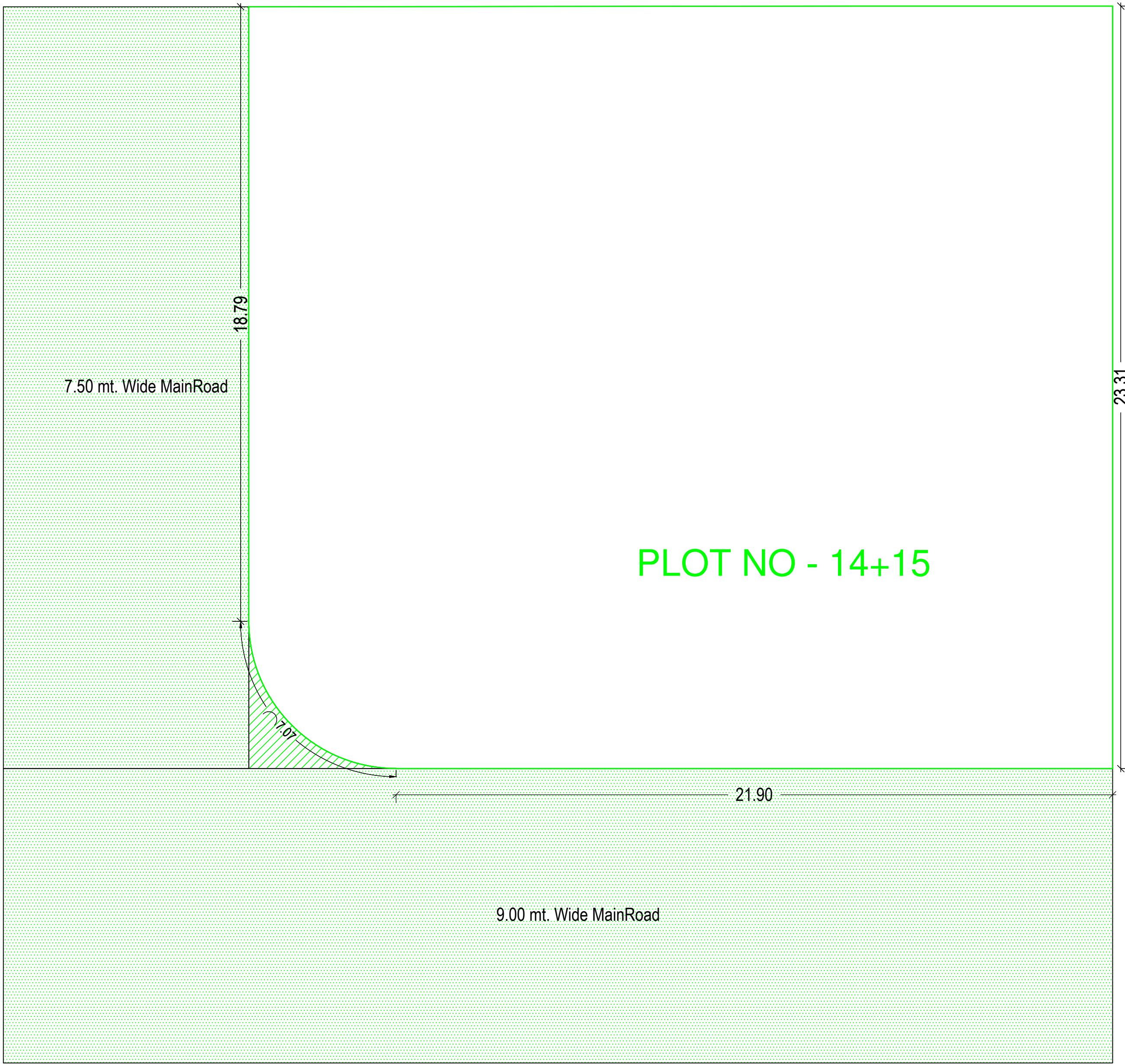
AFTER AMALGAMATION PLAN (Scale - 1:100)
