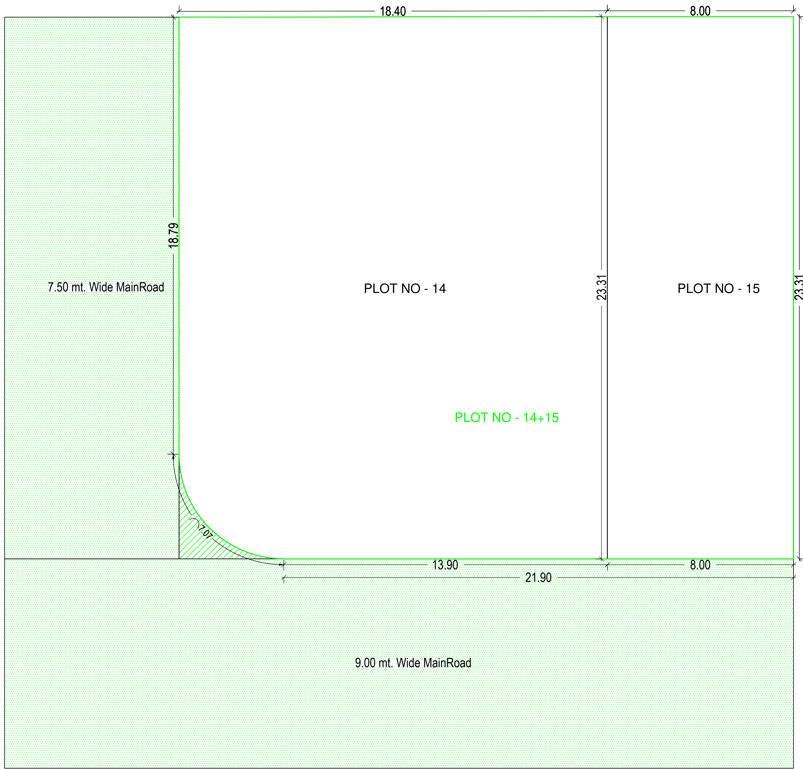
BEFORE AMALGAMATION PLAN (Scale - 1:100)
