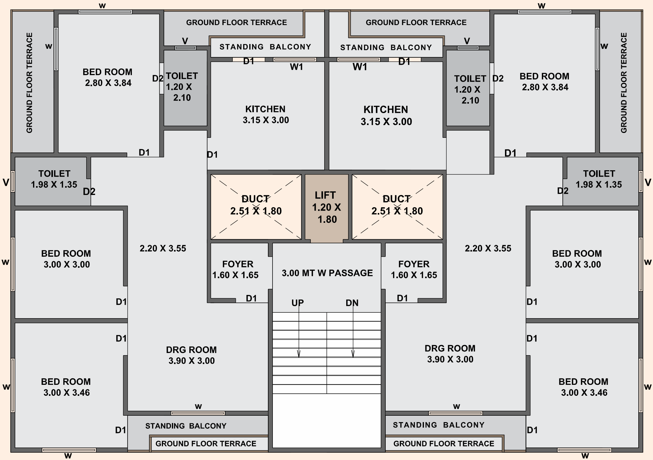
TYPICAL FLOOR
