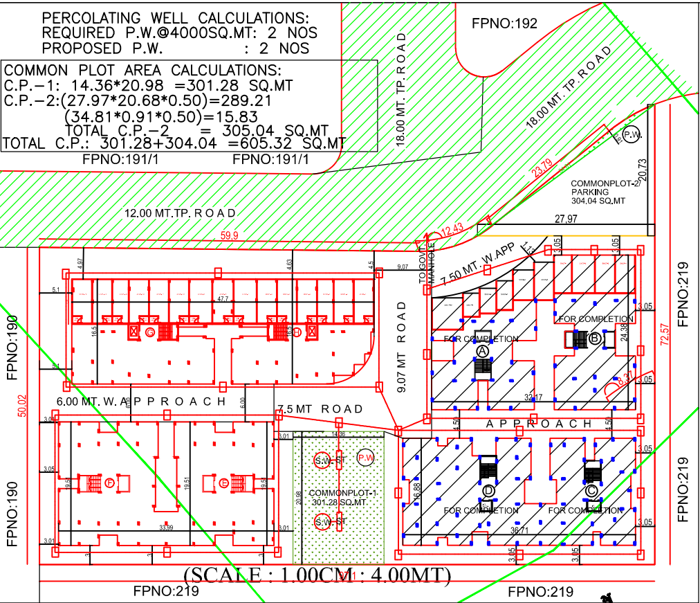
LAYOUT PLAN
