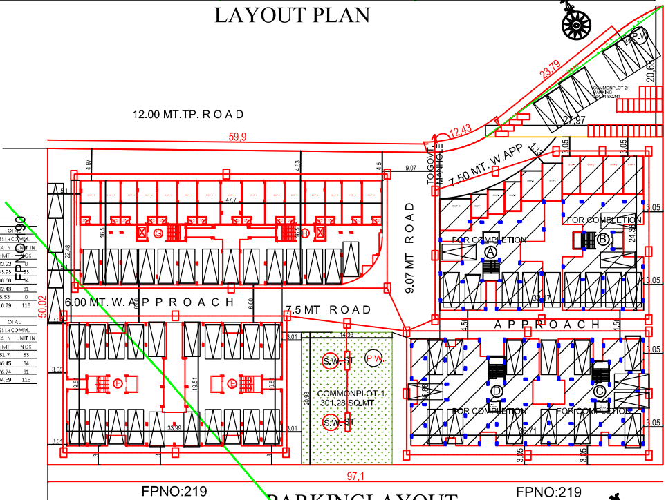
PARKING LAYOUT (SCALE : 1.00CM : 4.00MT)
