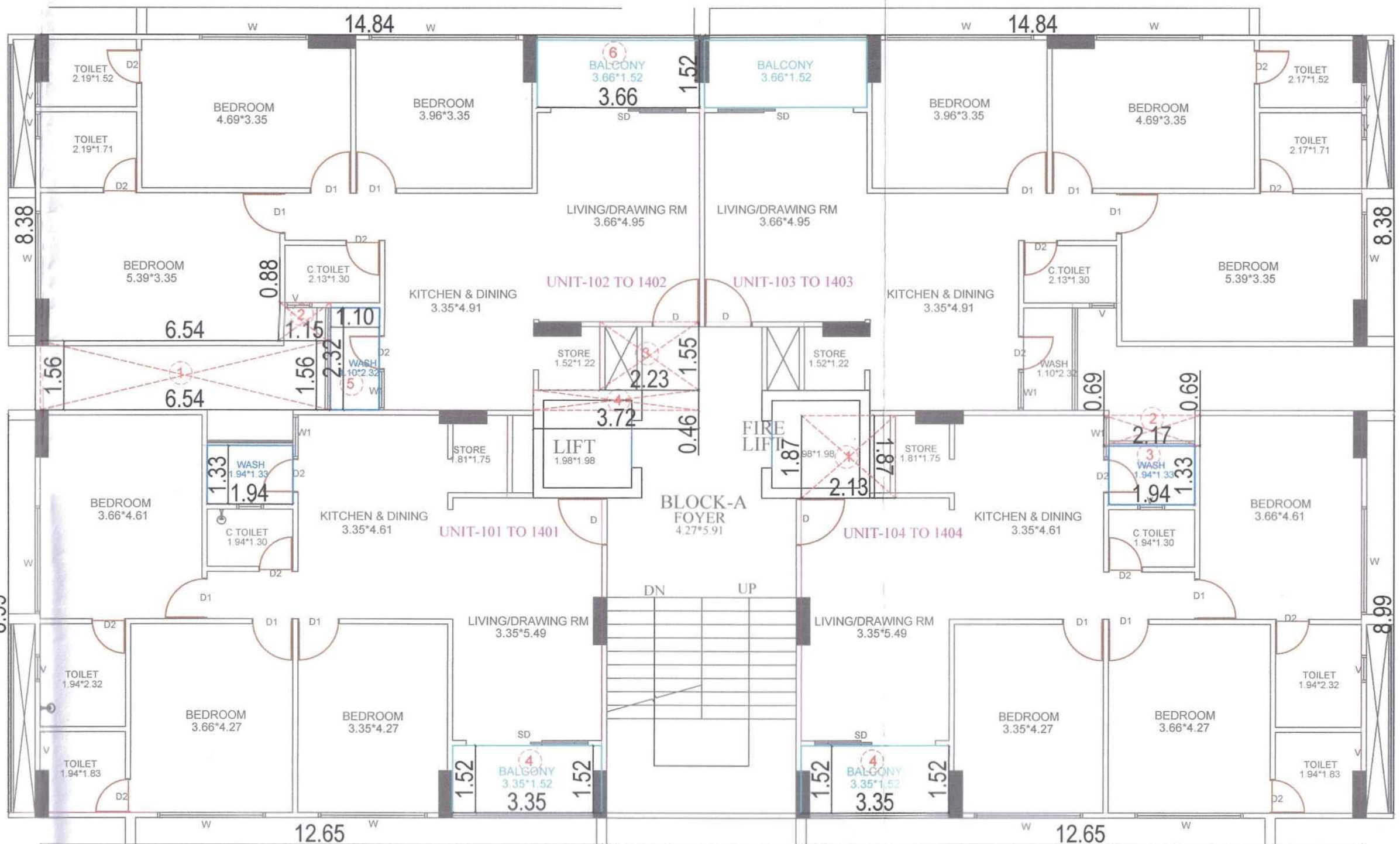
CARPET AREA CALCULATION SKETCH
