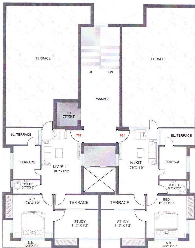
Seventh Floor Plan
