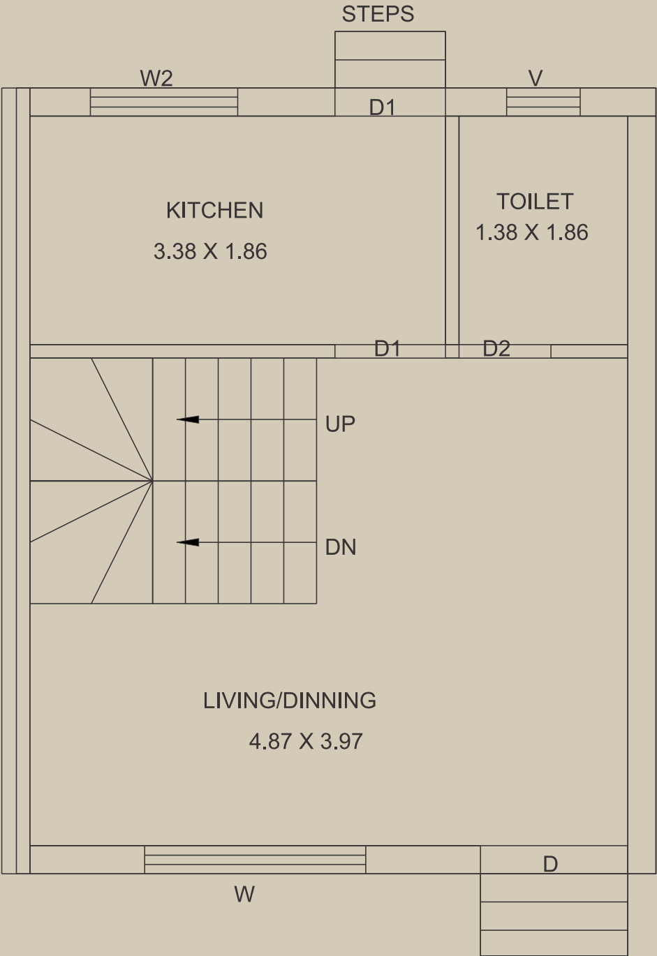
GROUND FLOOR
