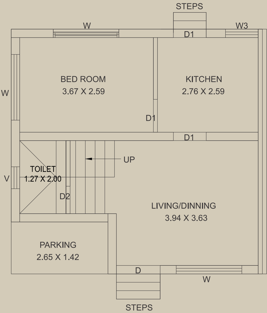
GROUND FLOOR
