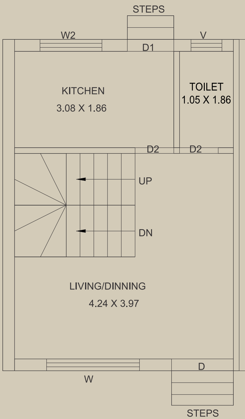
GROUND FLOOR
