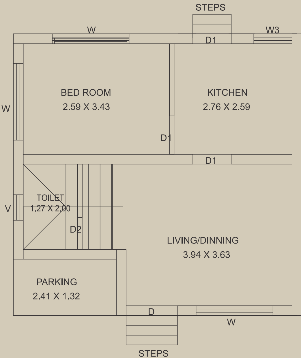
GROUND FLOOR
