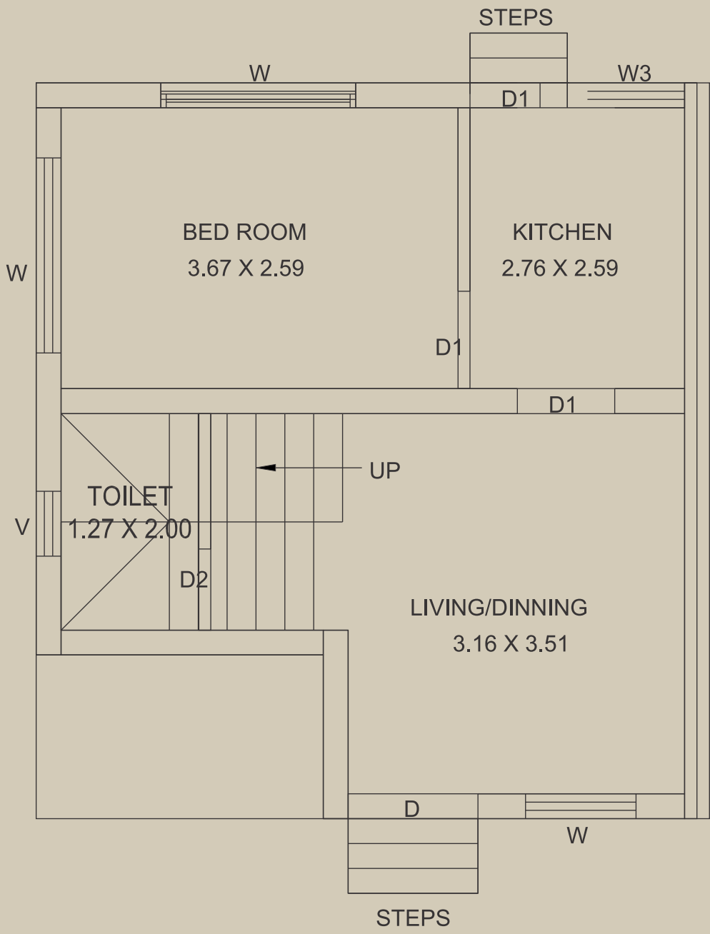
GROUND FLOOR
