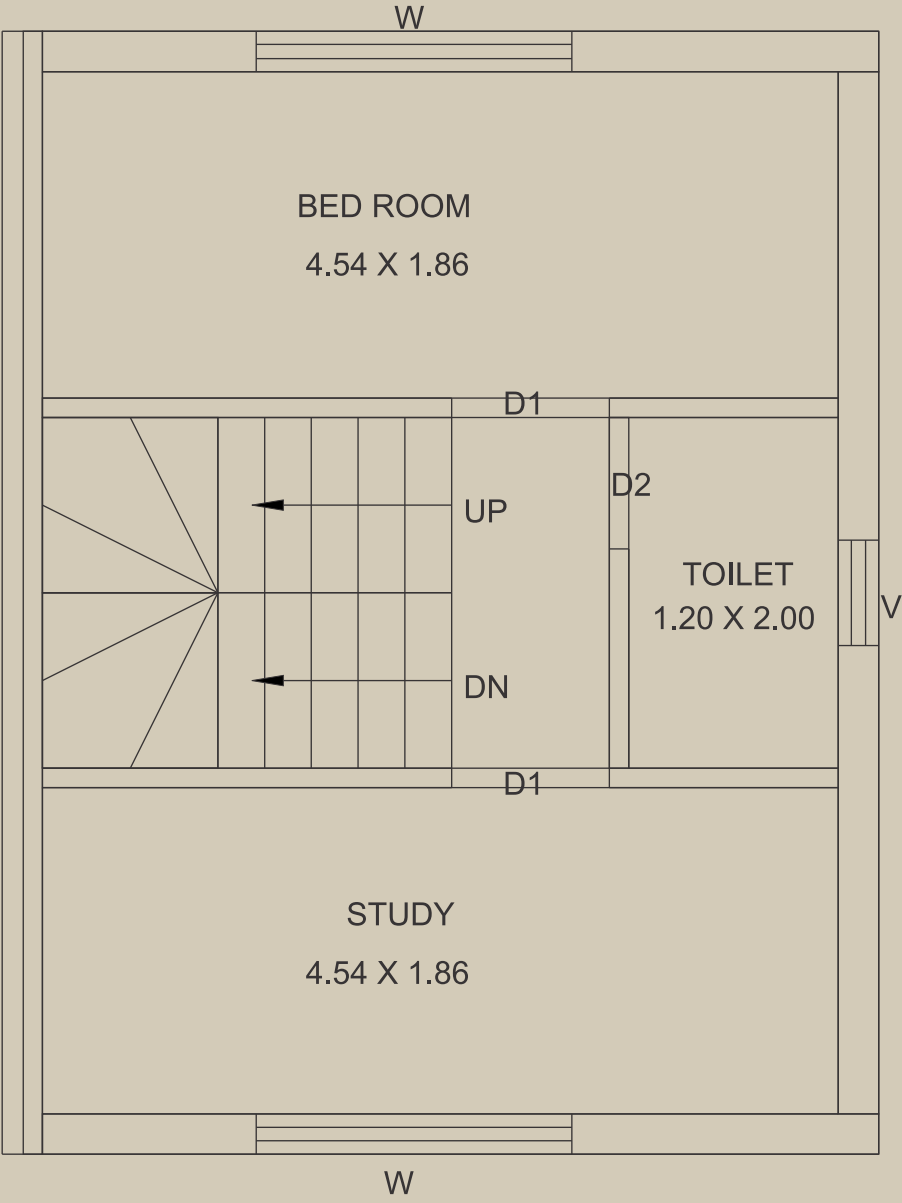
FIRST FLOOR
