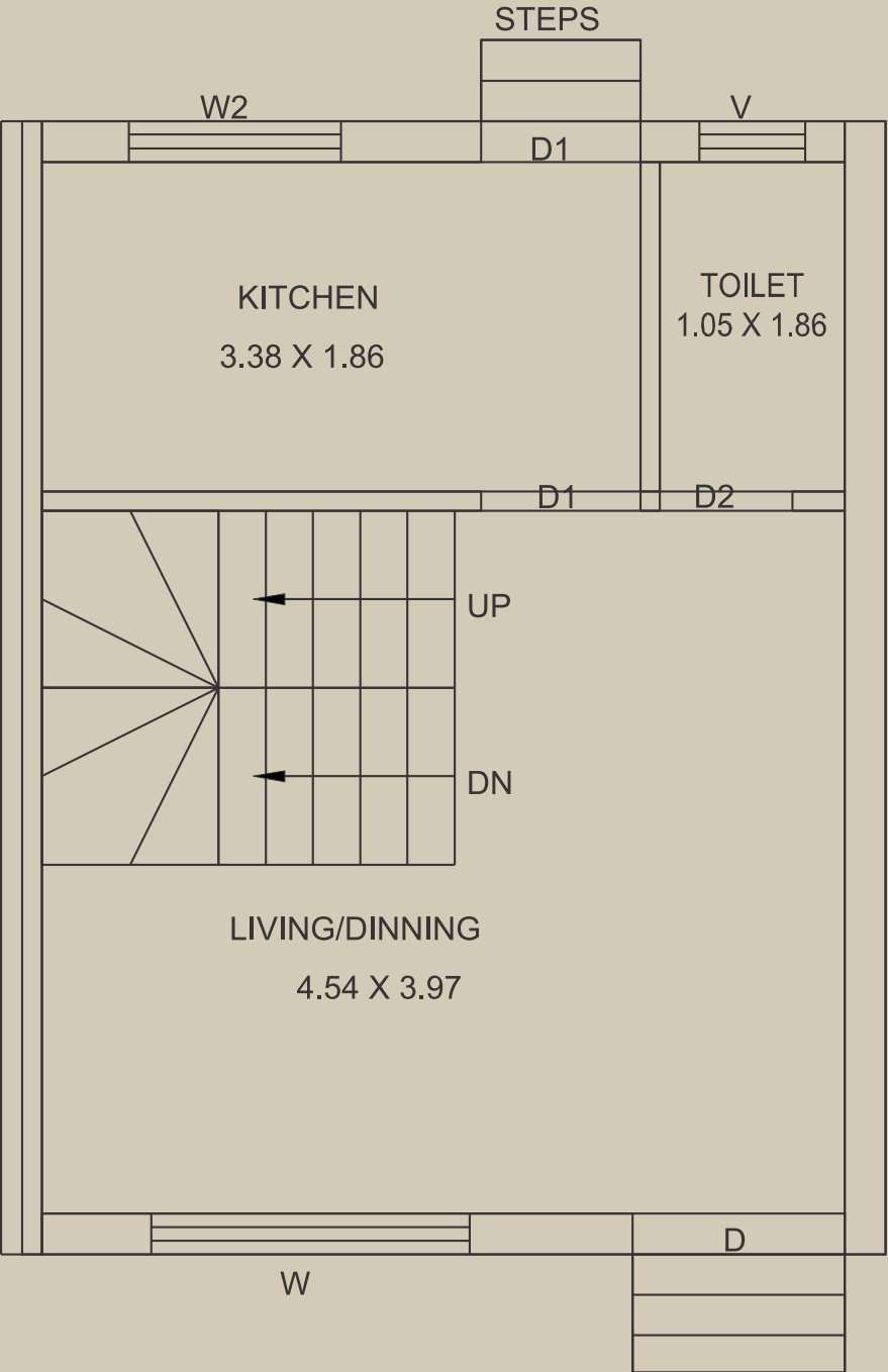
GROUND FLOOR
