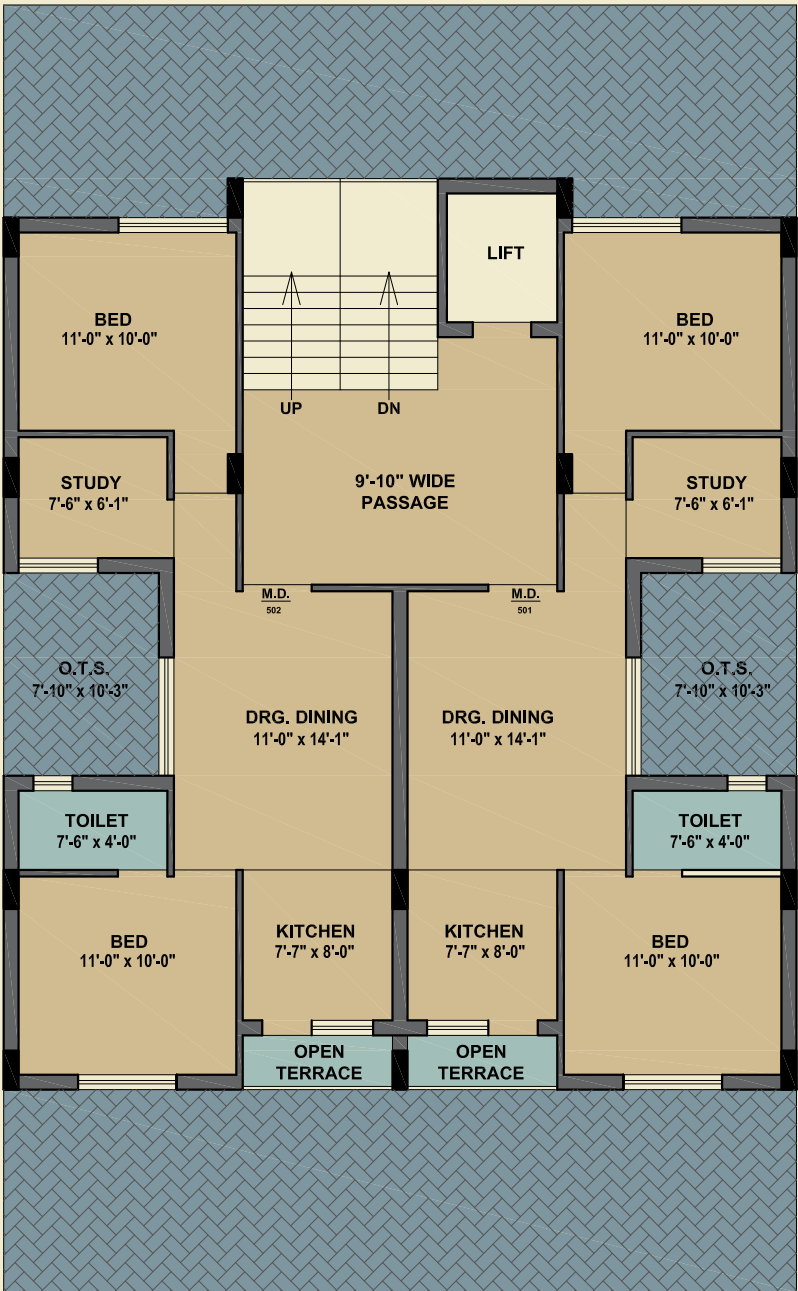
5th FLOOR
