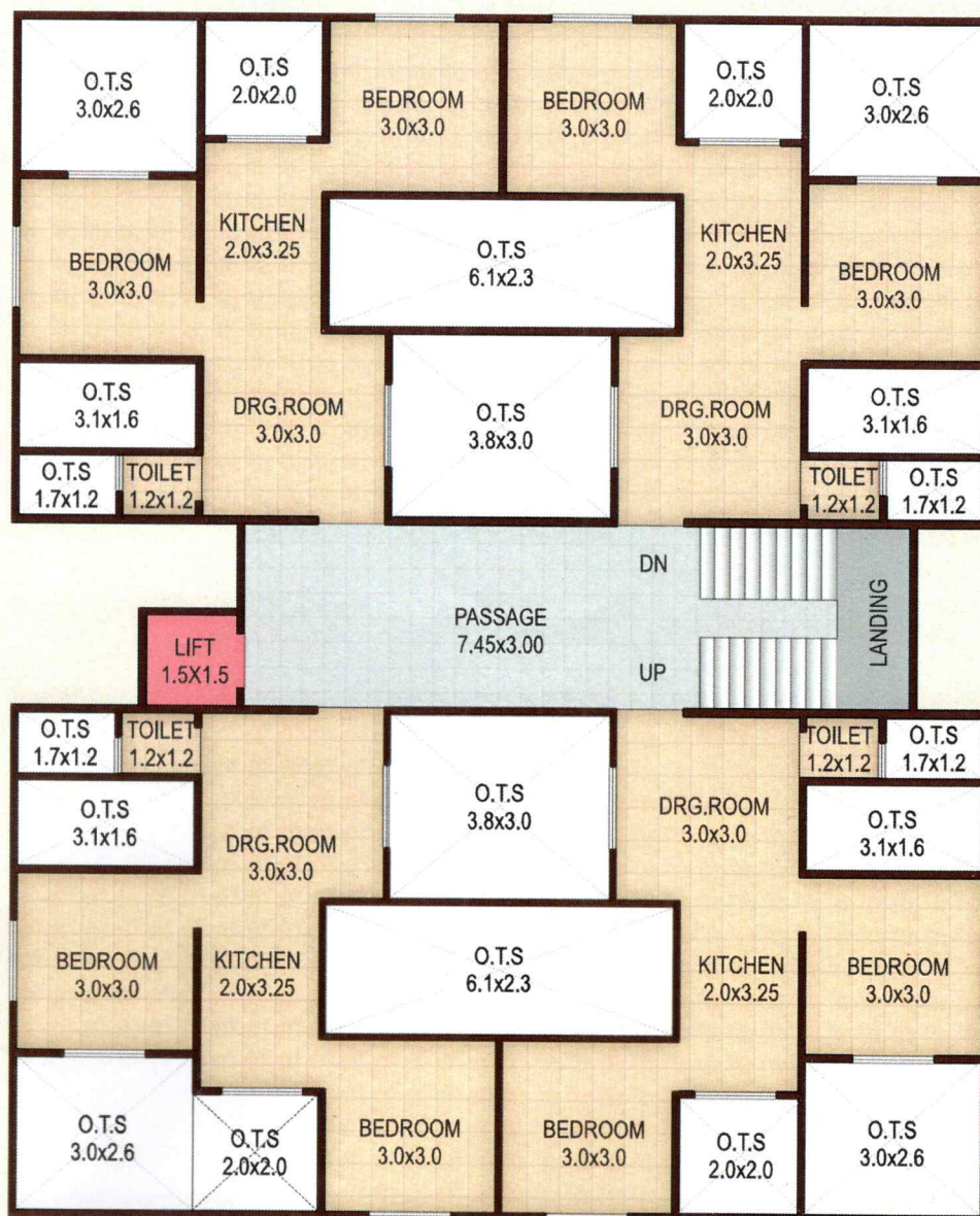
Typical Floor Tower A,C & D
