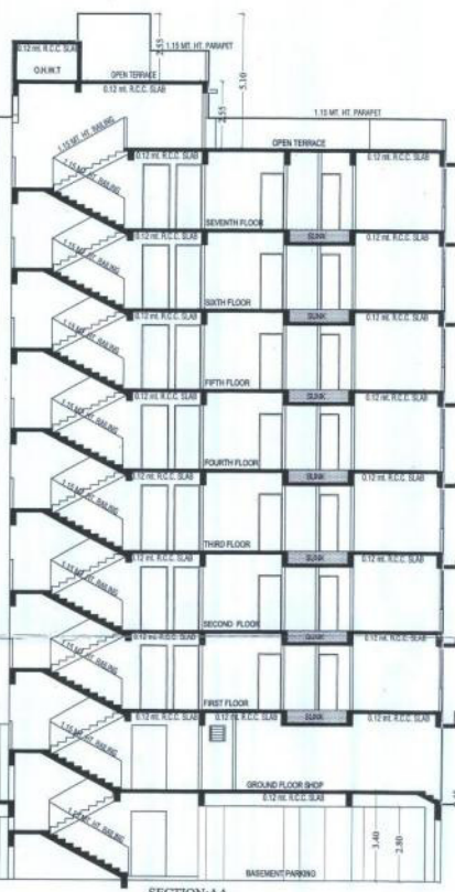
SECTION AA
