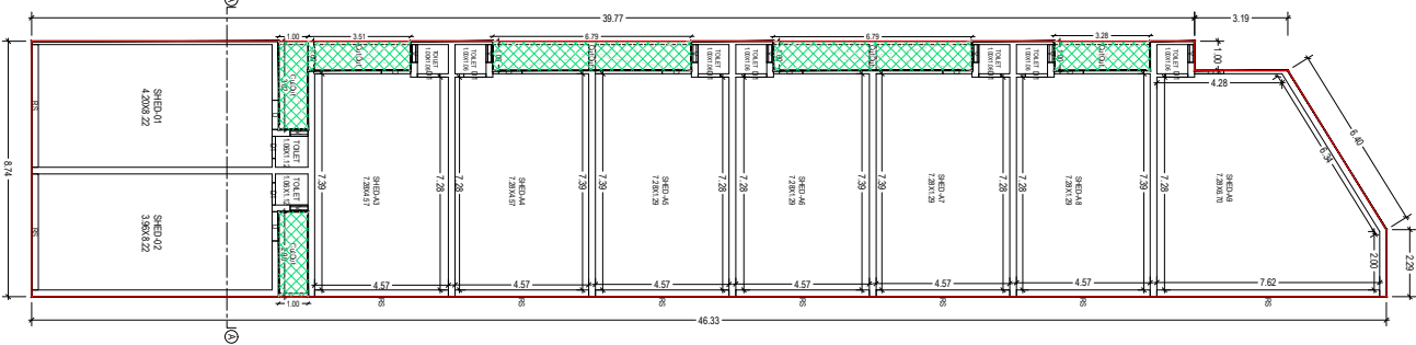
GROUND FLOOR PLAN (Proposed) (SCALE 1:100)
