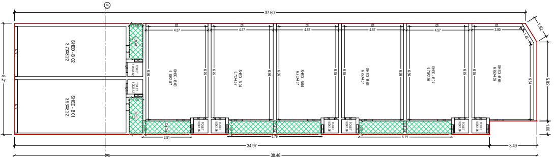
GROUND FLOOR PLAN (Proposed) (SCALE 1:100)
