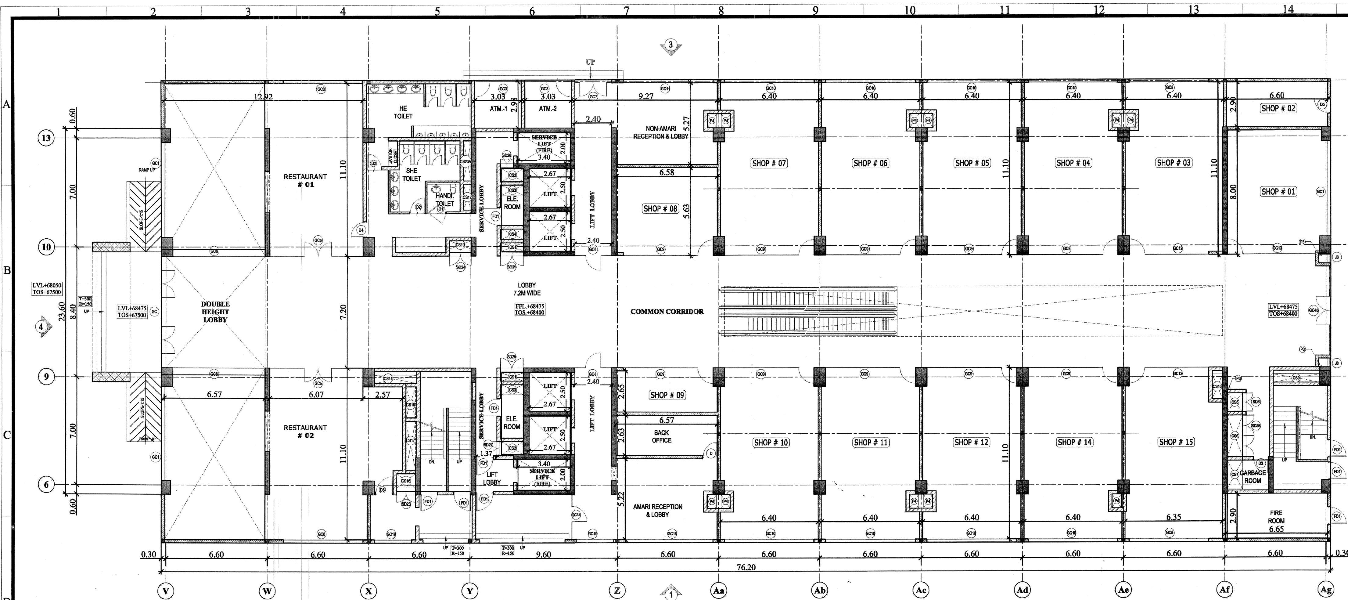
GROUND FLOOR PLAN T.O.S. LVL +68,400 F.F.L. +68,475
