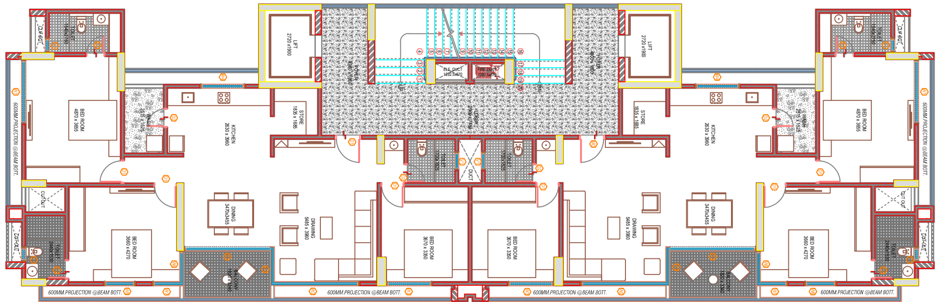
BUILDING B & C & D TYPICAL FLOOR PLAN
