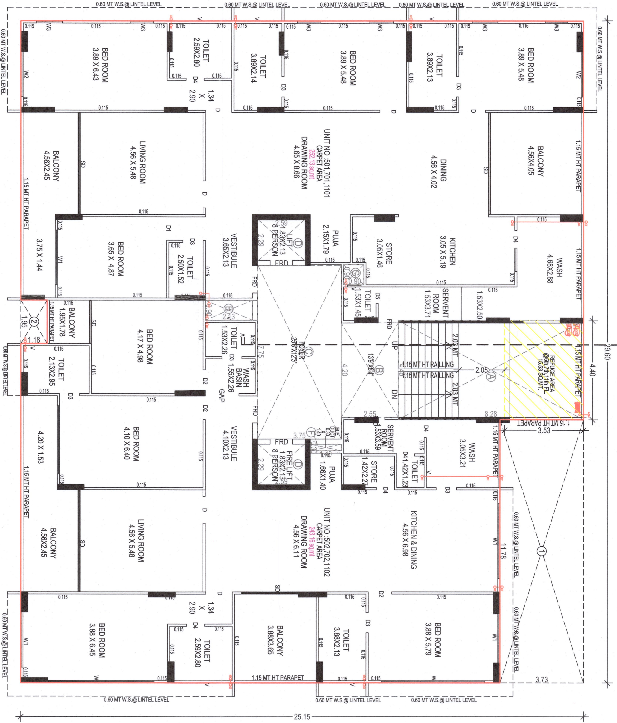
REFUGE FLOOR PLAN (8th, 7th, 11th)
