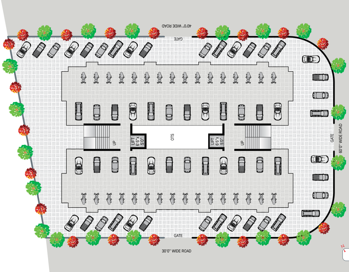
PARKING LAYOUT PLAN
