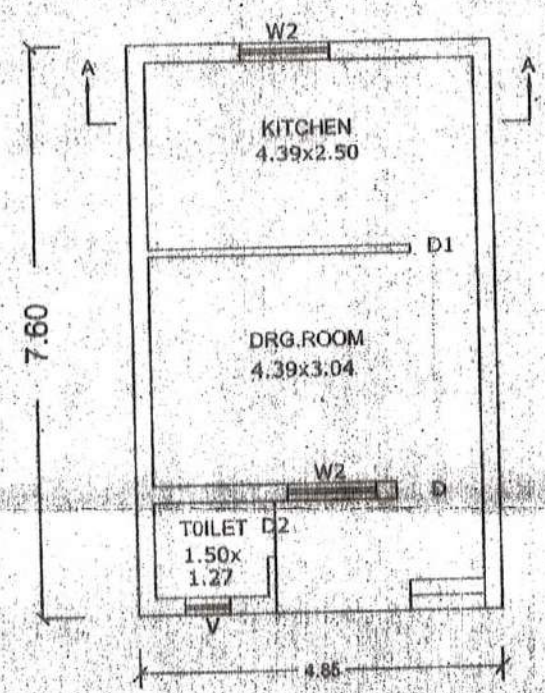
C.F. & F.F. PLAN SCALE - 1:100
