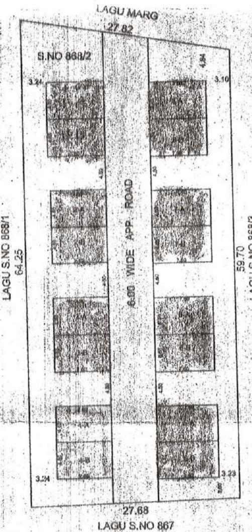
LAY-OUT PLAN SCALE = 1.0 CM = 5.0 MT
