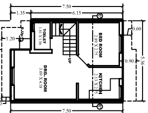
GROUND FL. PLAN B.U.P. Area: 38.13 X 13 = 457.56 Sq.mt. F.S.I. Area: 37.50 X 13 = 451.08 Sq.mt.
