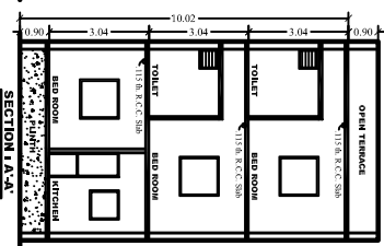
TYPE I-C FIRST FL. PLAN F.S.I. Area: 47.00 X 13 = 605.08 Sq.mt.
