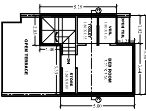
TYPE C SECOND FL. PLAN F.S.I. Area: 27.55 X 13 = 358.20 Sq.mt.
