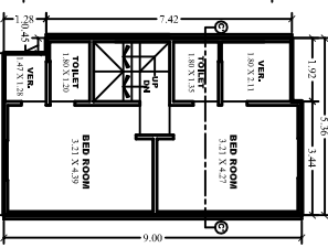
TYPE I-C FIRST FL. PLAN F.S.I. Area: 47.00 X 13 = 605.08 Sq.mt.
