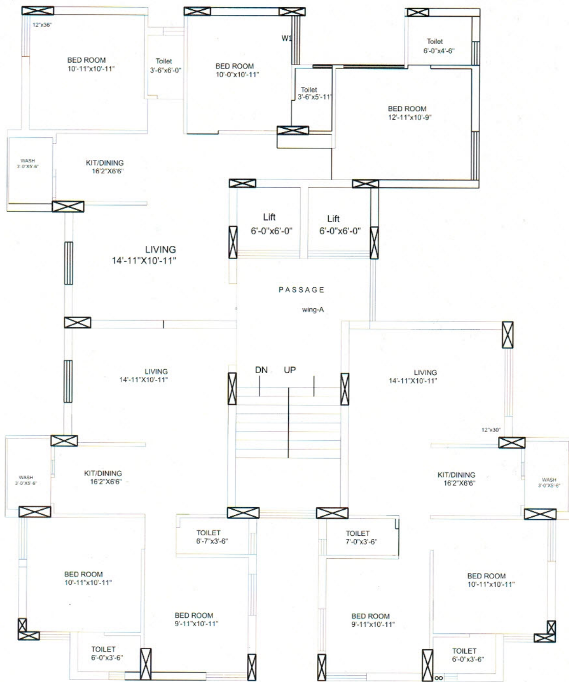
24 MT WIDE ROAD TYPICAL FLOOR PLAN ( 1 TO 12)
