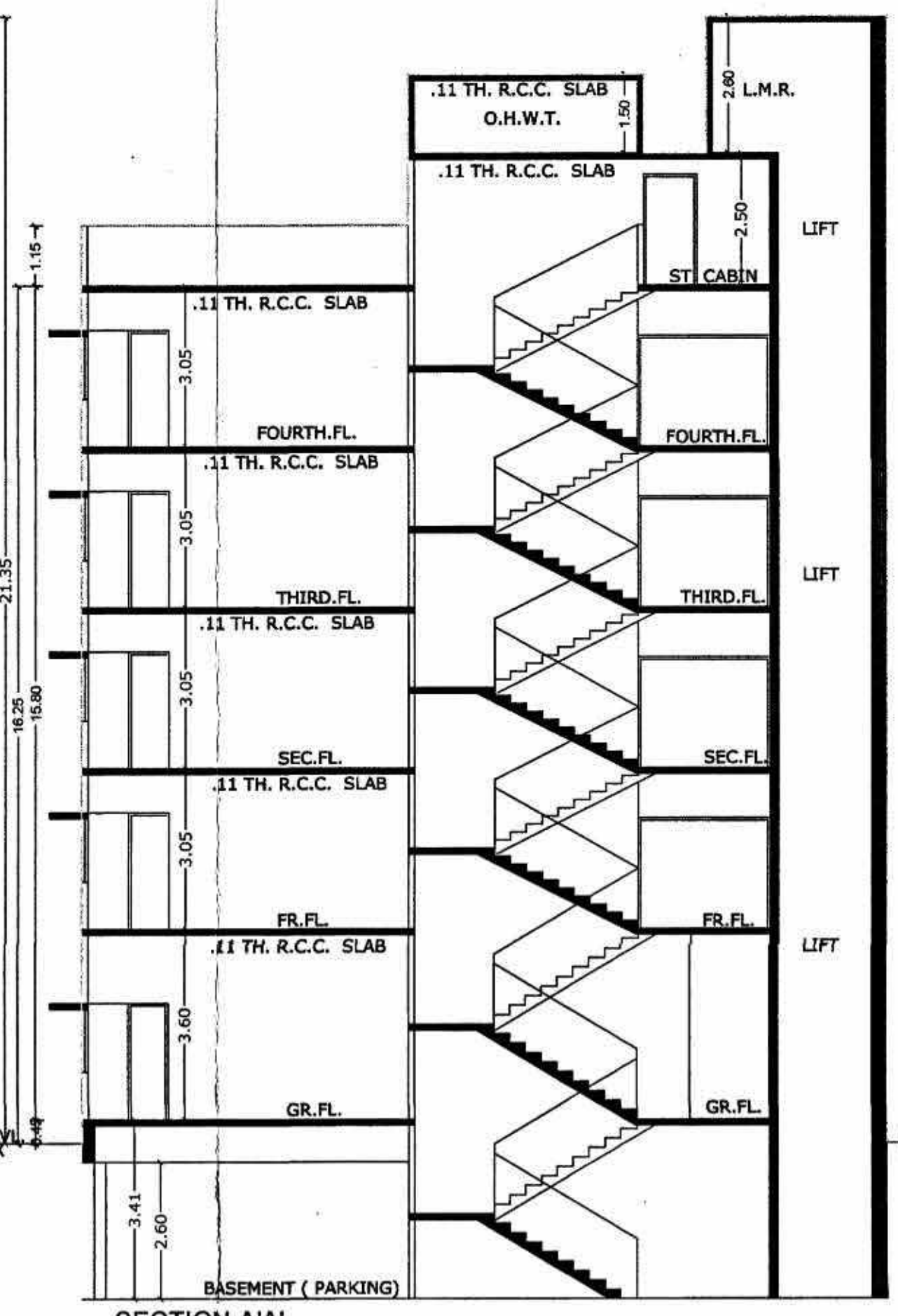
SECTION-AA'
