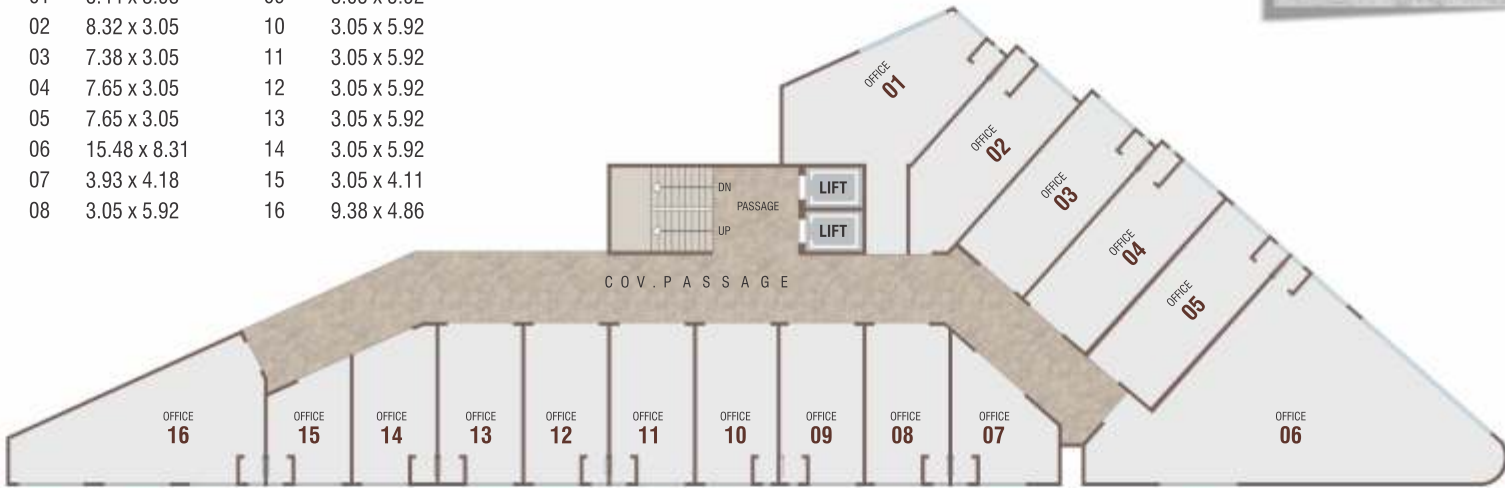
4 TH & 5 TH Floor Plan
