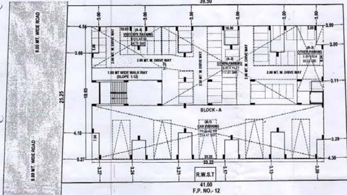
PARKING LAYOUT PLAN SCALE: 1 CM = 2.00 MT
