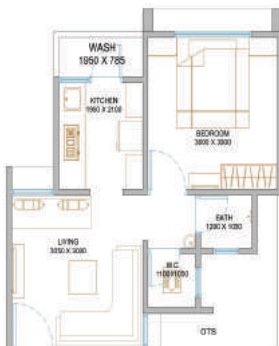
EWS UNIT PLAN
