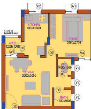
EWS UNIT PLAN
