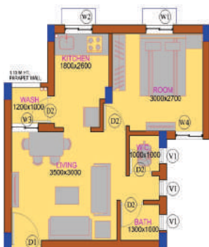
EWS UNIT PLAN
