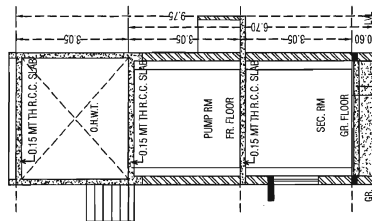
SECTION - XX
