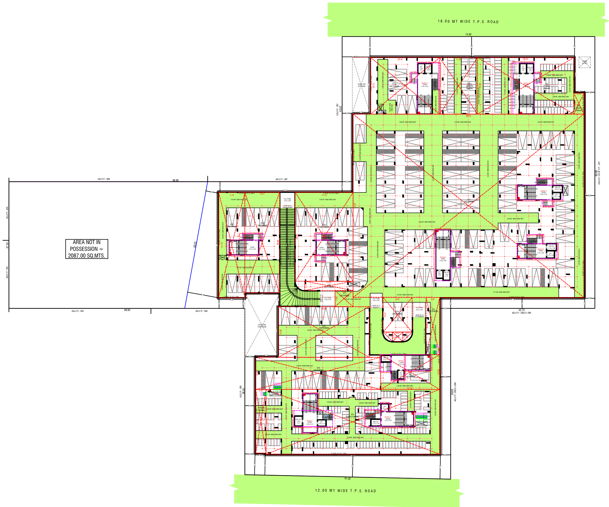
1ST BASEMENT PLAN
