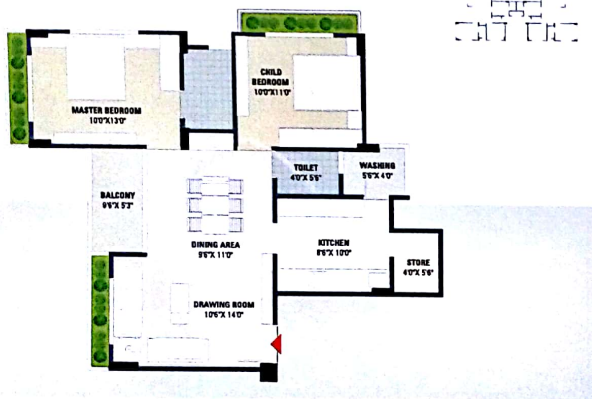
B & C-BLOCK UNIT PLAN - 2 BHK
