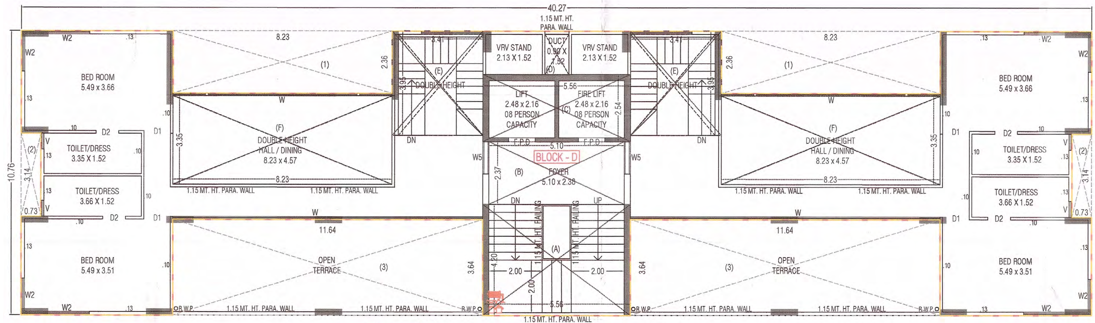
Block D - 801 & 802(Lower Level Plan) 8th Floor
