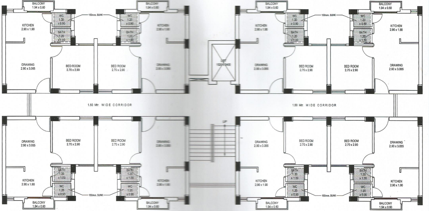
Floor Plan
