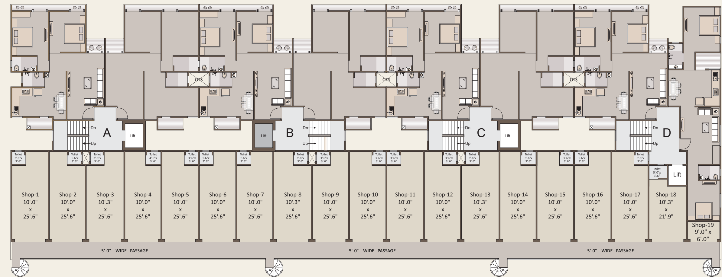
Tower-A,B,C,D FIRST FLOOR PLAN
