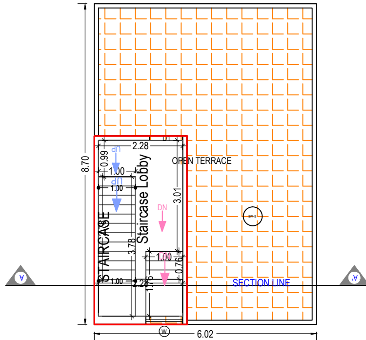
TERRACE FLOOR PLAN (Proposed) (SCALE 1:100)
