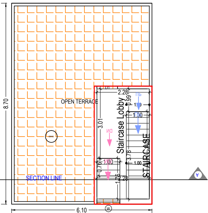
TERRACE FLOOR PLAN (Proposed) (SCALE 1:100)
