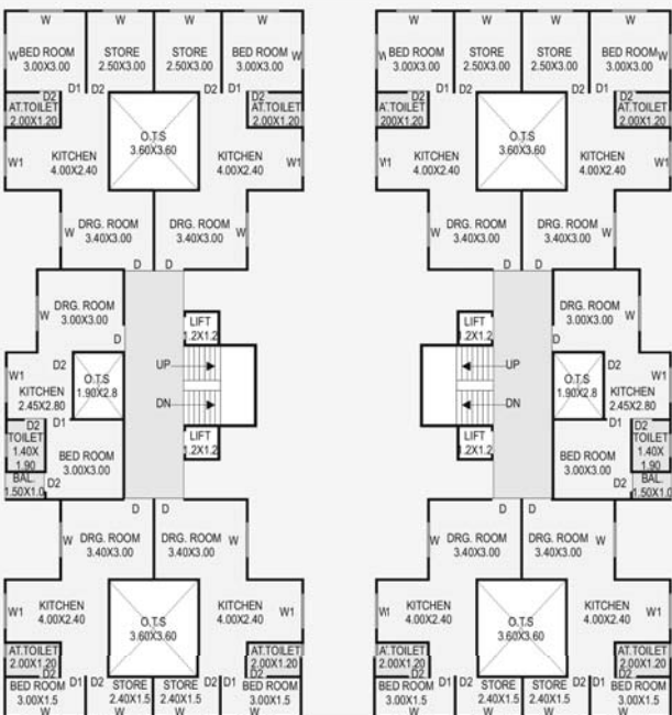
2nd TO 6th FLOOR PLAN
