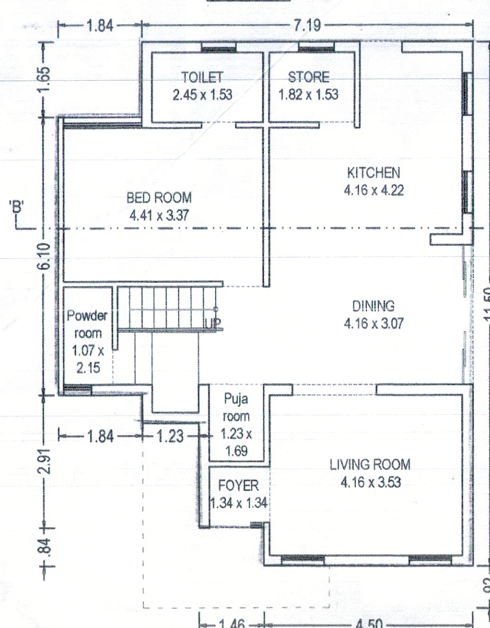
TYPE - B GROUND FLOOR PLAN BUILT UP AREA = 88.80 SQ.MT. = 88.80 X 30 = 2664.00 SQ.MT.
