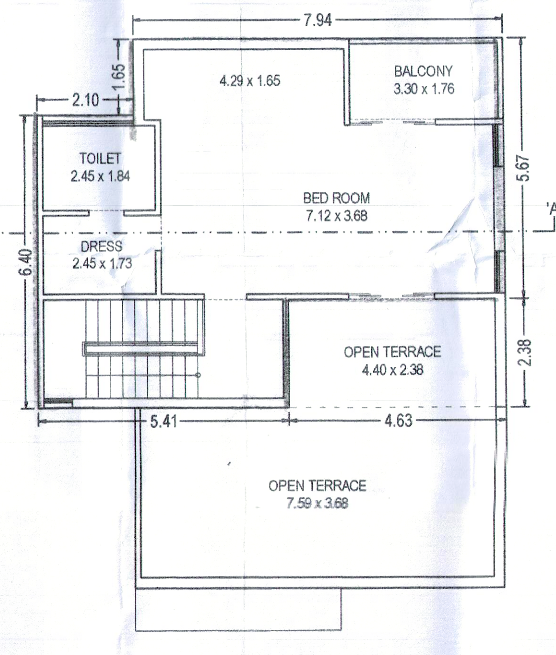
TYPE - A SECOND FLOOR PLAN BUILT UP AREA = 66.32 SQ.MT. = 66.32 X 23 = 1525.36 SQ.MT.
