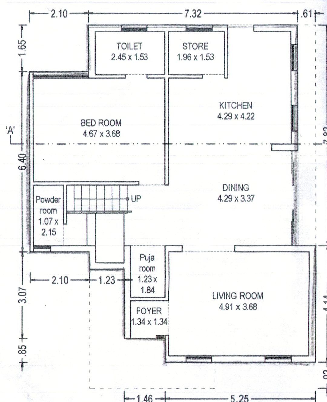
TYPE - A GROUND FLOOR PLAN BUILT UP AREA = 98.29 SQ.MT. = 98.29 X 23 = 2260.67 SQ.MT.
