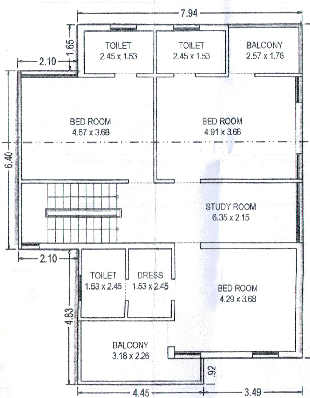
TYPE - A FIRST FLOOR PLAN BUILT UP AREA = 112.46 SQ.MT. = 112.46 X 23 = 2586.58 SQ.MT.
