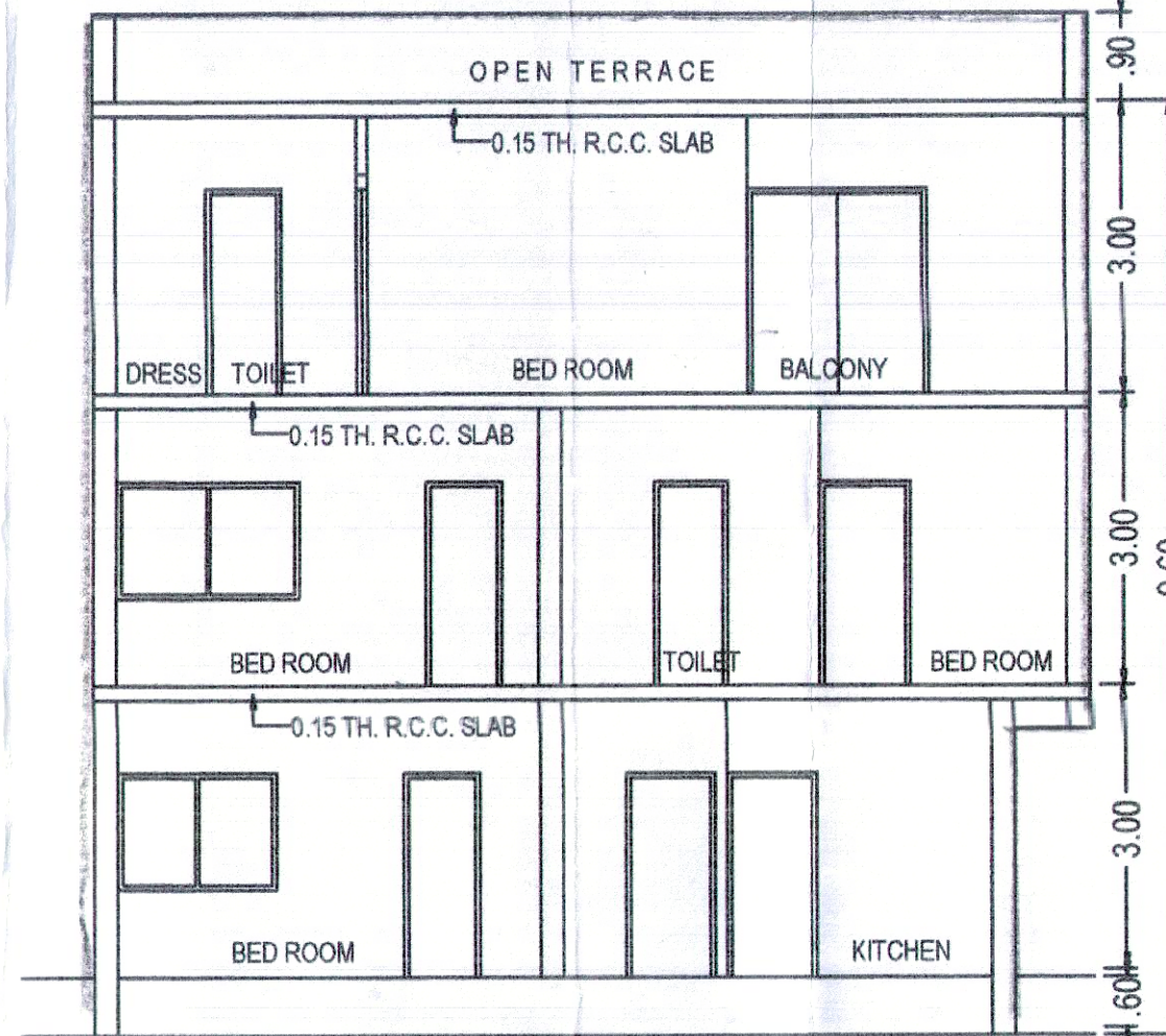
SECTION = 'A-A'
