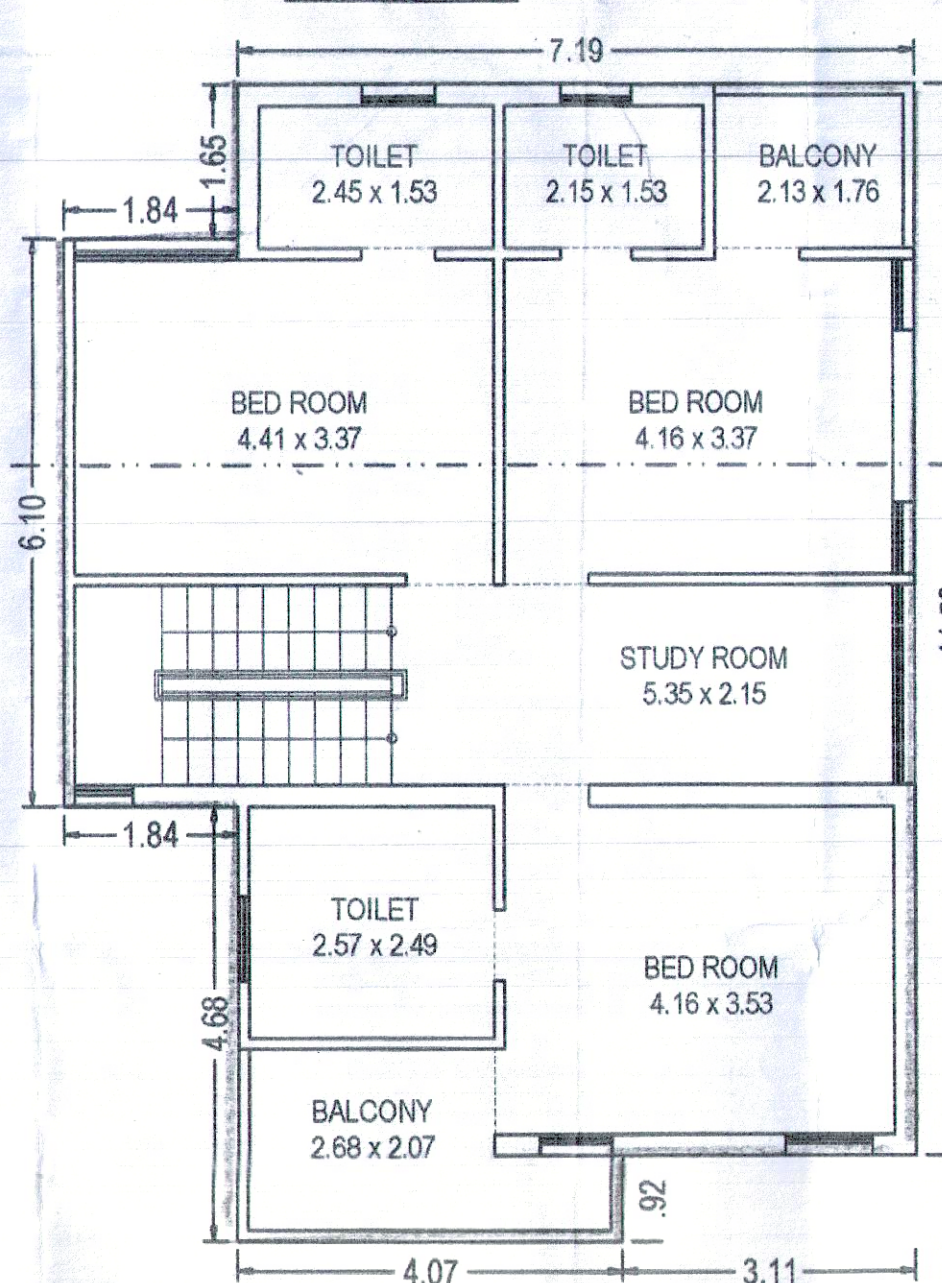
TYPE - B FIRST FLOOR PLAN BUILT UP AREA = 97.63 SQ.MT. = 97.63 X 30 = 2928.90 SQ.MT.
