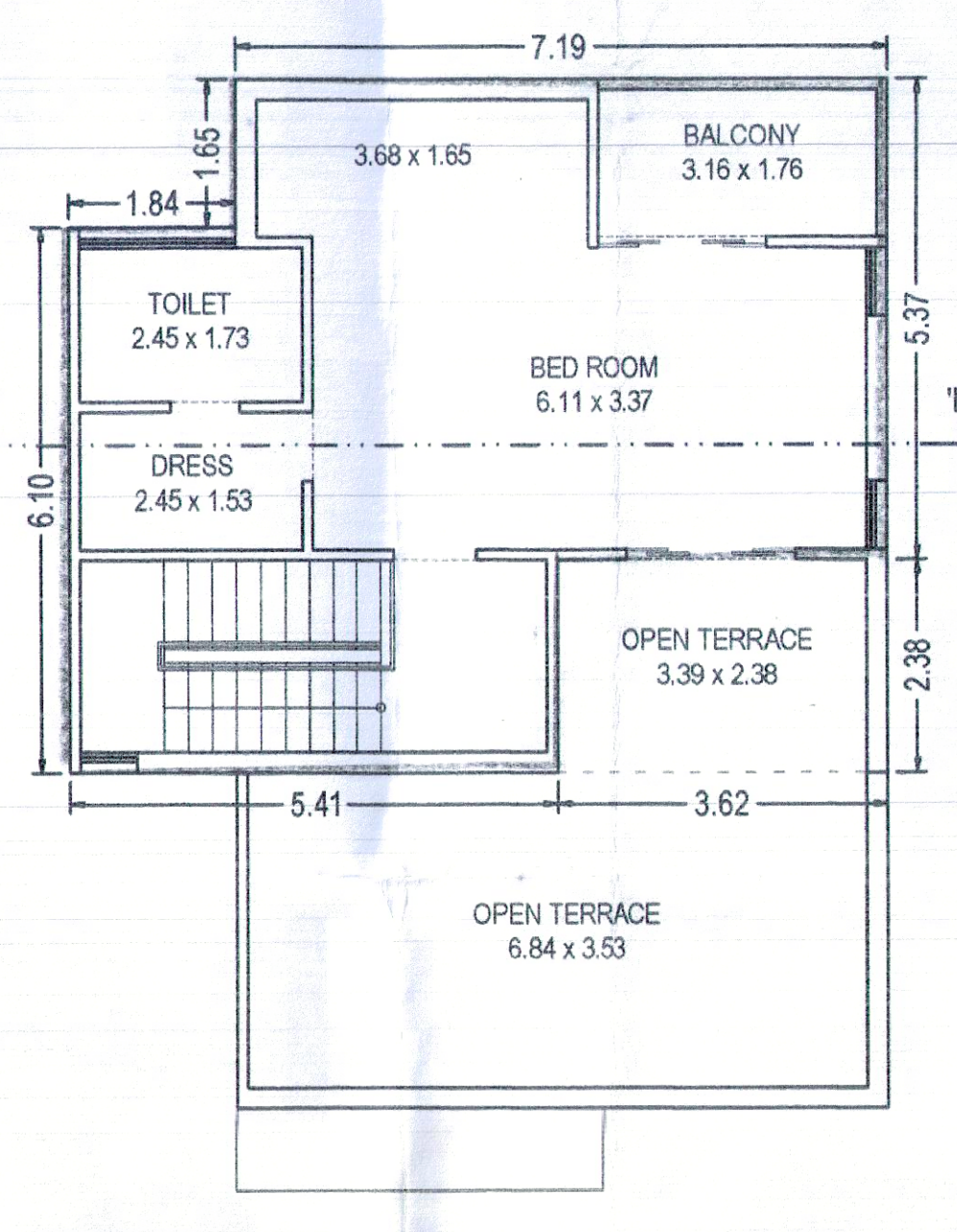
TYPE - B SECOND FLOOR PLAN BUILT UP AREA = 58.26 SQ.MT. = 58.26 X 30 = 1747.80 SQ.MT.
