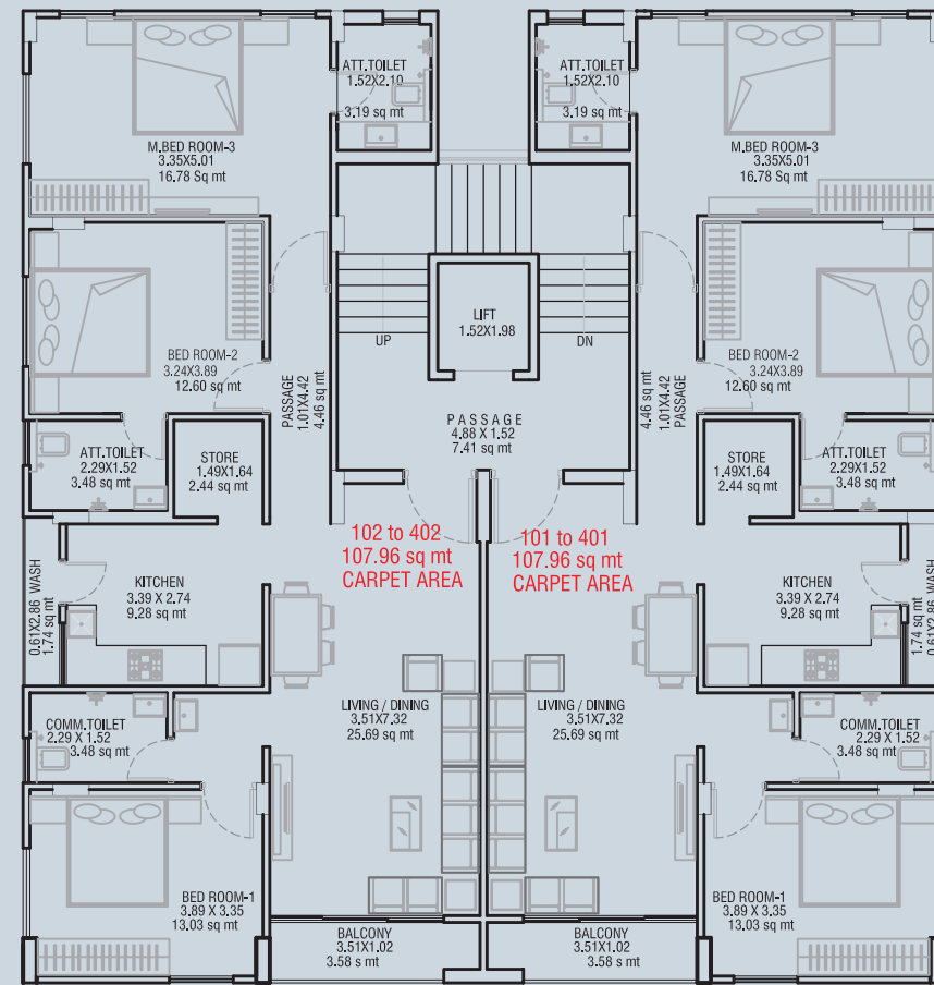
TYPICAL FLOOR PLAN(1st. TO 4th.)
