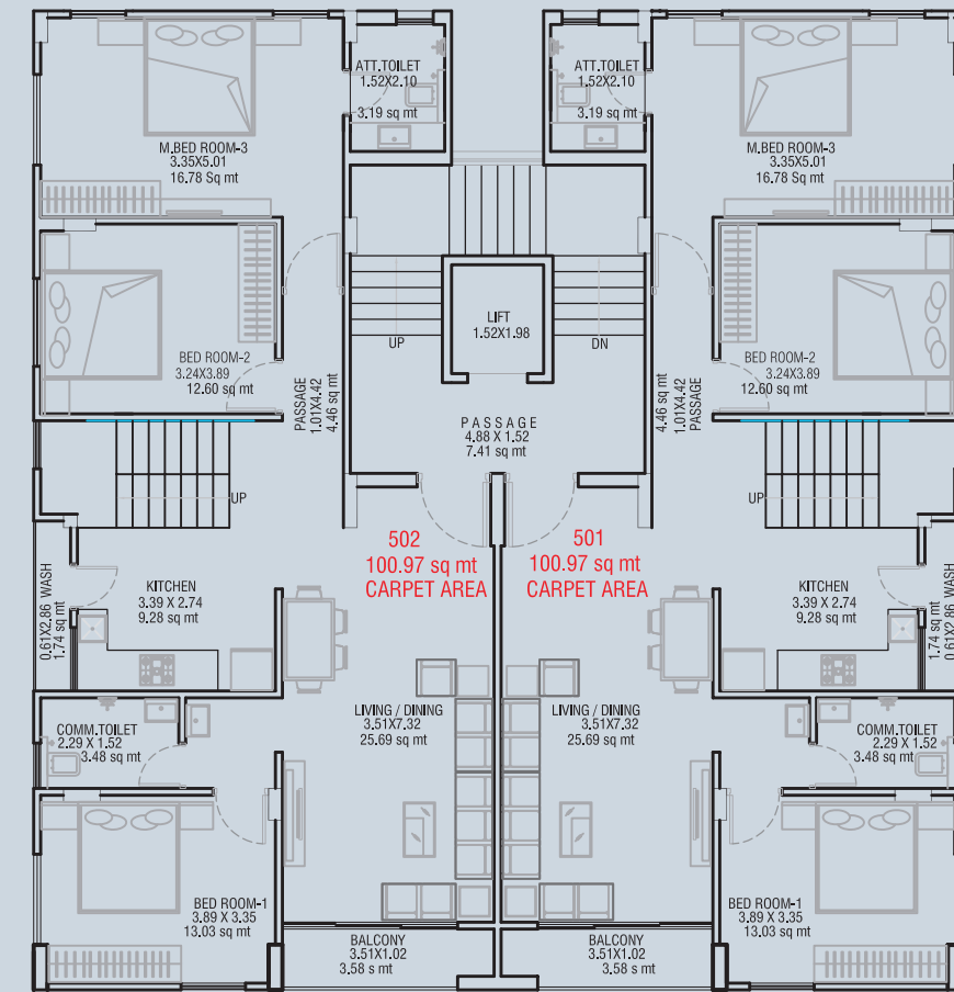
5th FLOOR PLAN
