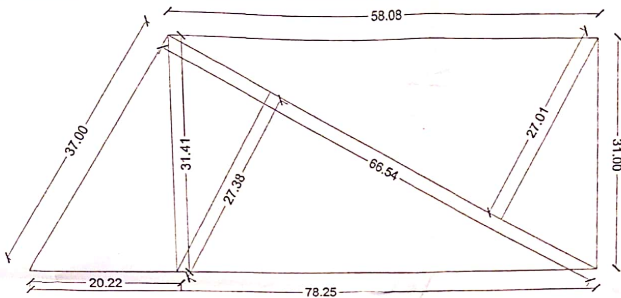
PLOT LAY OUT PLAN SCALE :- 1.00CM = 5.00MT
