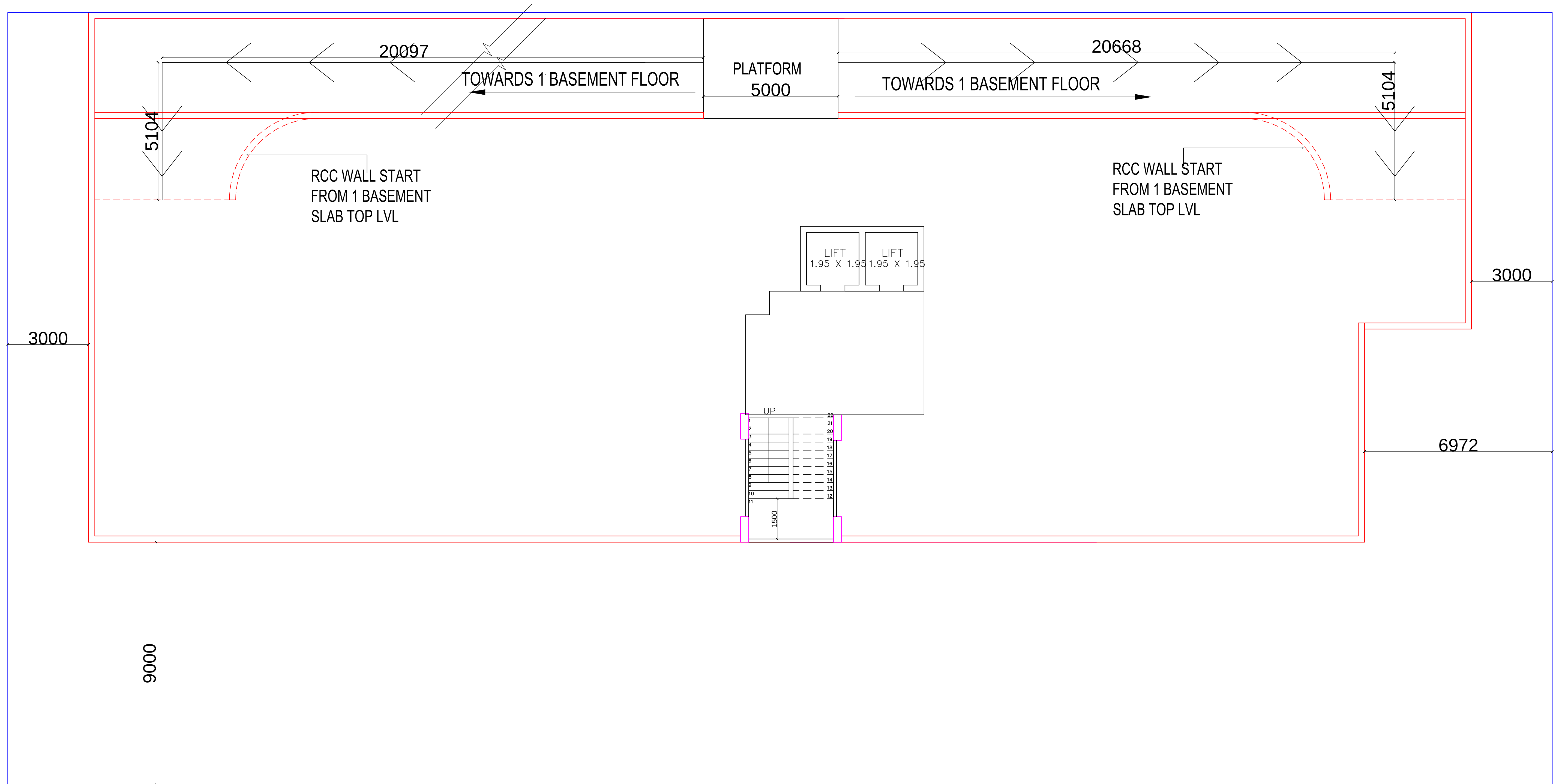
2 BASEMENT FLOOR PLAN
