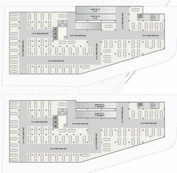
1 st BASEMENT
