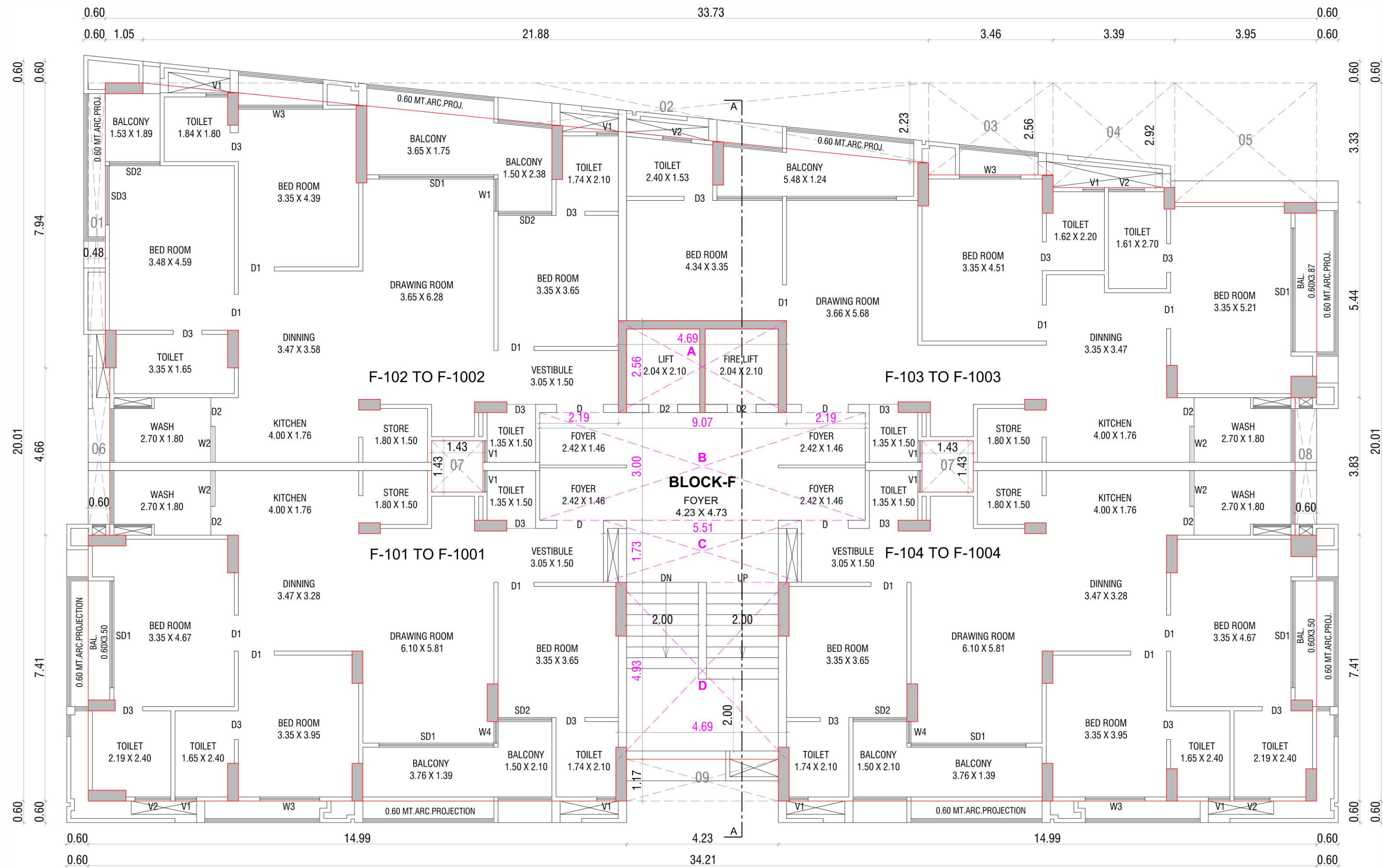
TYPICAL FLOOR PLAN (1ST TO 10TH FLOOR)
