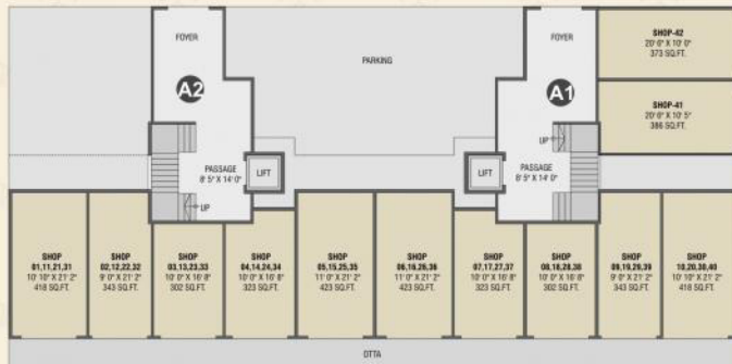
SHOP TYPICAL PLAN_A1, A2, B1, B2, C1, C2, D1, D2
