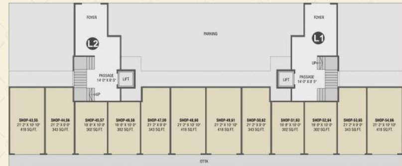
SHOP TYPICAL PLAN_K1, K2, L1, L2
