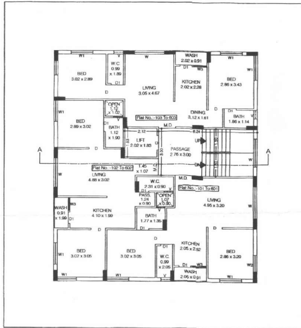
PROP. FIRST TO SIX FLOOR PLAN (SCALE: 1:100)
