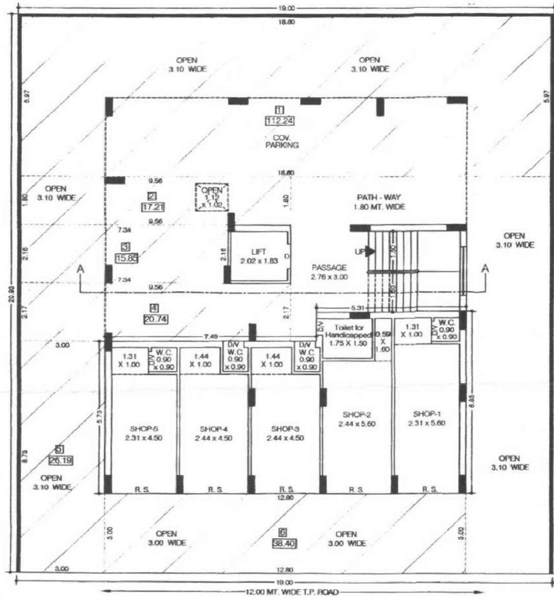
PROP. GROUND FLOOR PLAN (SCALE: 1:100)
