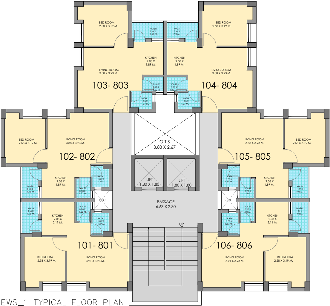
EWS_1 TYPICAL FLOOR PLAN
