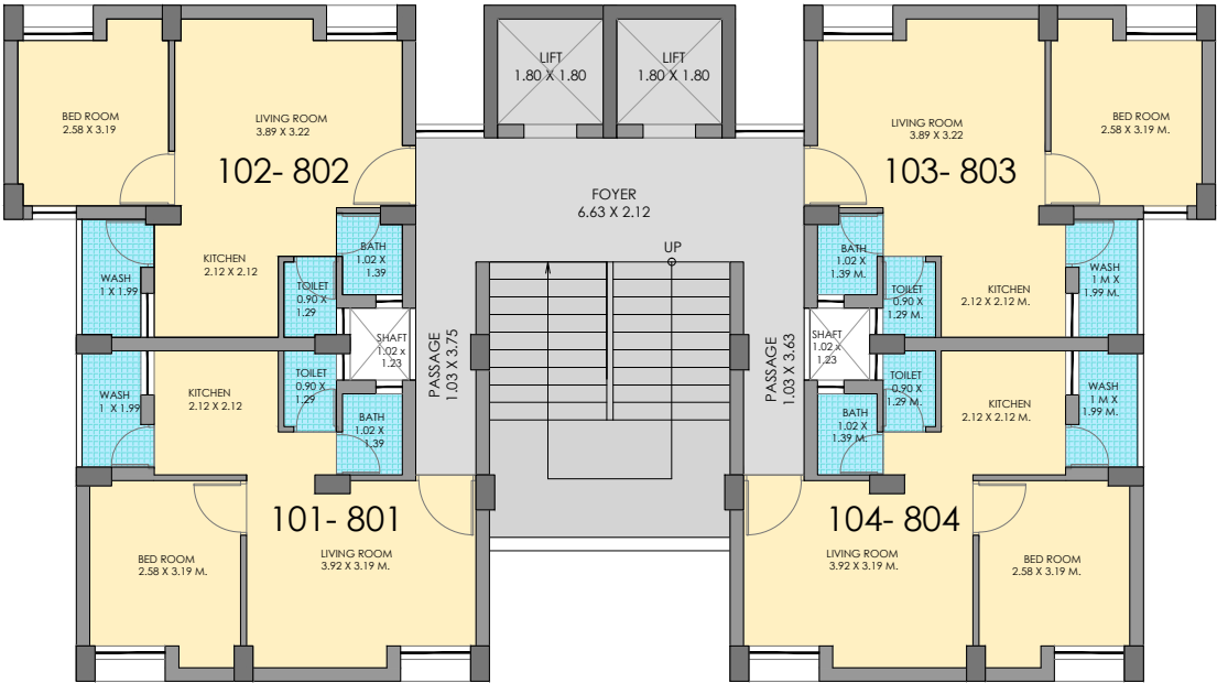
EWS_1 TYPICAL FLOOR PLAN
