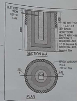
SOAK PIT DETAIL
