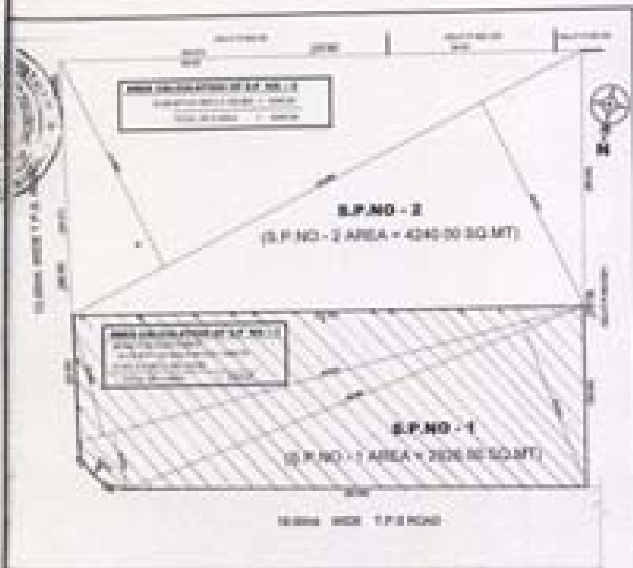
PROPOSED SUB DIVISION LAYOUT PLAN
