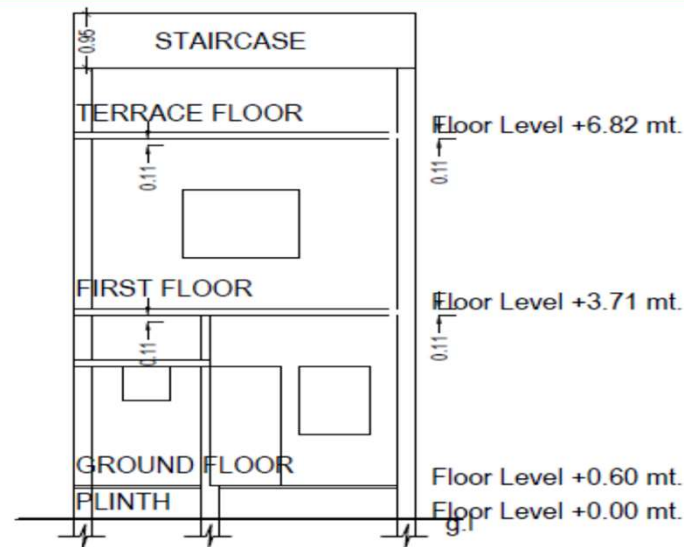
SECTION -AT-A-A
