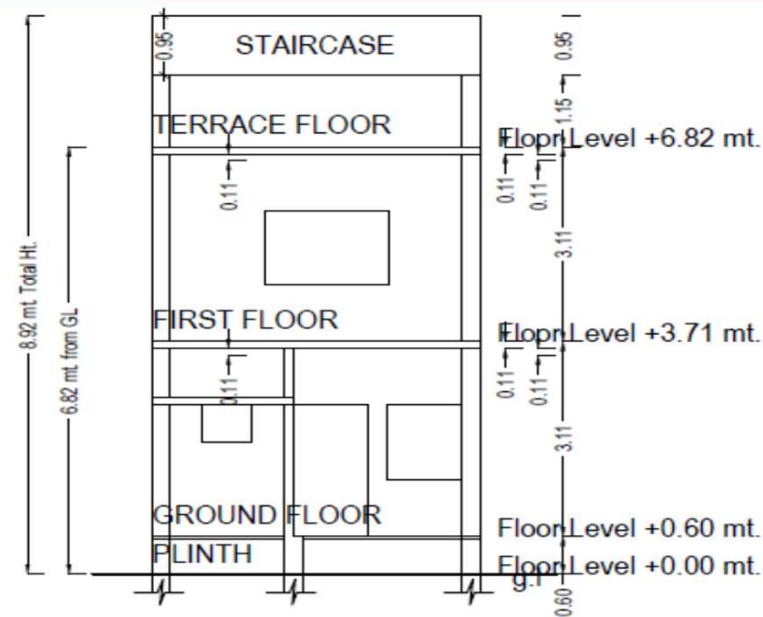
SECTION -AT-C-C
