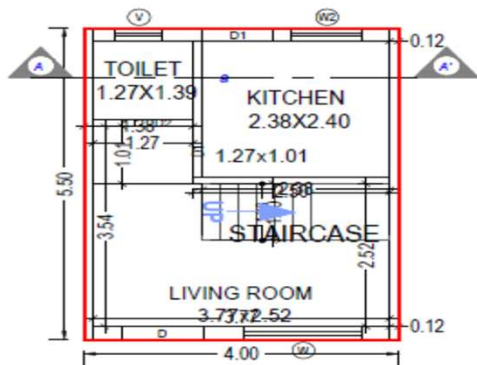
GROUND FLOOR PLAN (Proposed) (SCALE 1:100)
