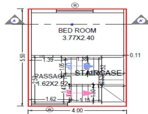
FIRST FLOOR PLAN (Proposed) (SCALE 1:100)
