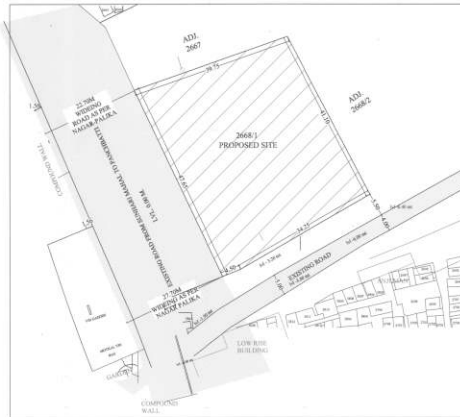
KEY PLAN (SCALE:- 1 CM = 4.00 MT)
