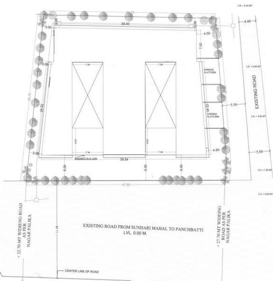
LAYOUT PLAN. (scale:-1 cm = 2.00 mt)
