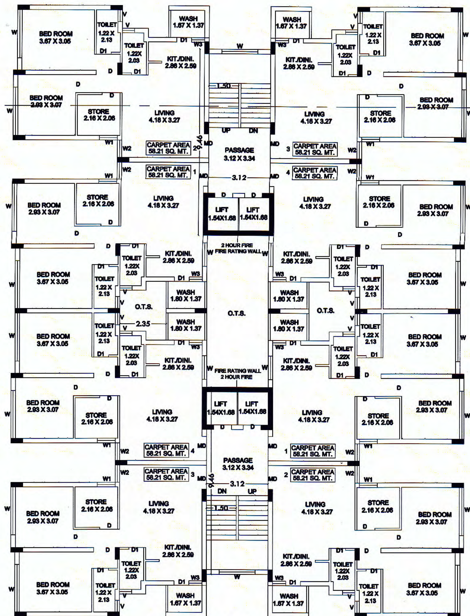
1st TO 8th FLOOR PLAN TOWER A & B, C & D, E & F
